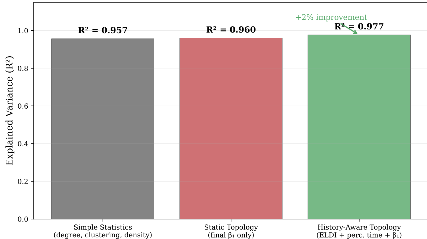
Figure 5: Model Comparison History-Aware Features Outperform Static Descriptors
