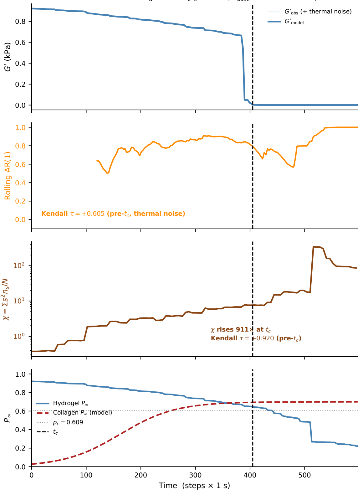
Gel-Sol Transition Signatures ( p_c = 0.609 , k_{\text{base}} = 0.001 \text{ s}^{-1} \text{ nM}^{-1} )
