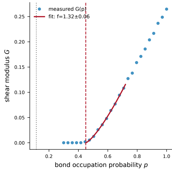
N=1720 (box=12) rigidity onset
