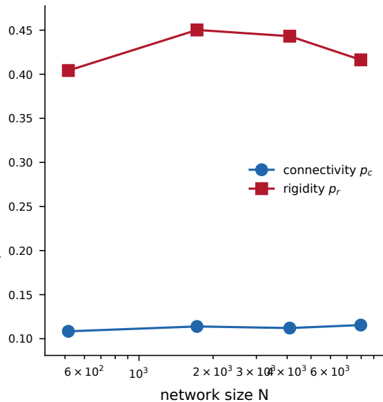
Thresholds vs. system size
