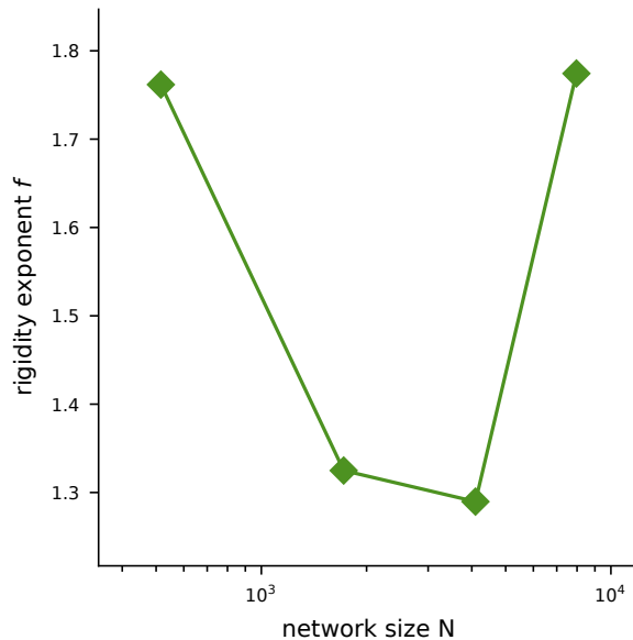
Rigidity exponent vs. system size
