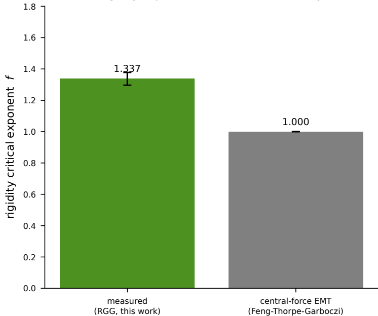
Measured rigidity exponent vs. central-force theory
