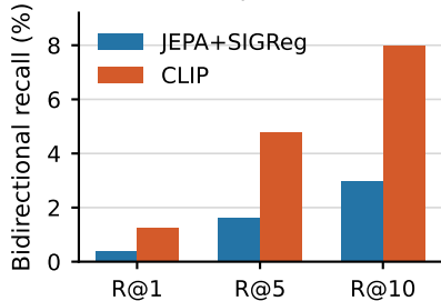
(a) Exact pair retrieval
