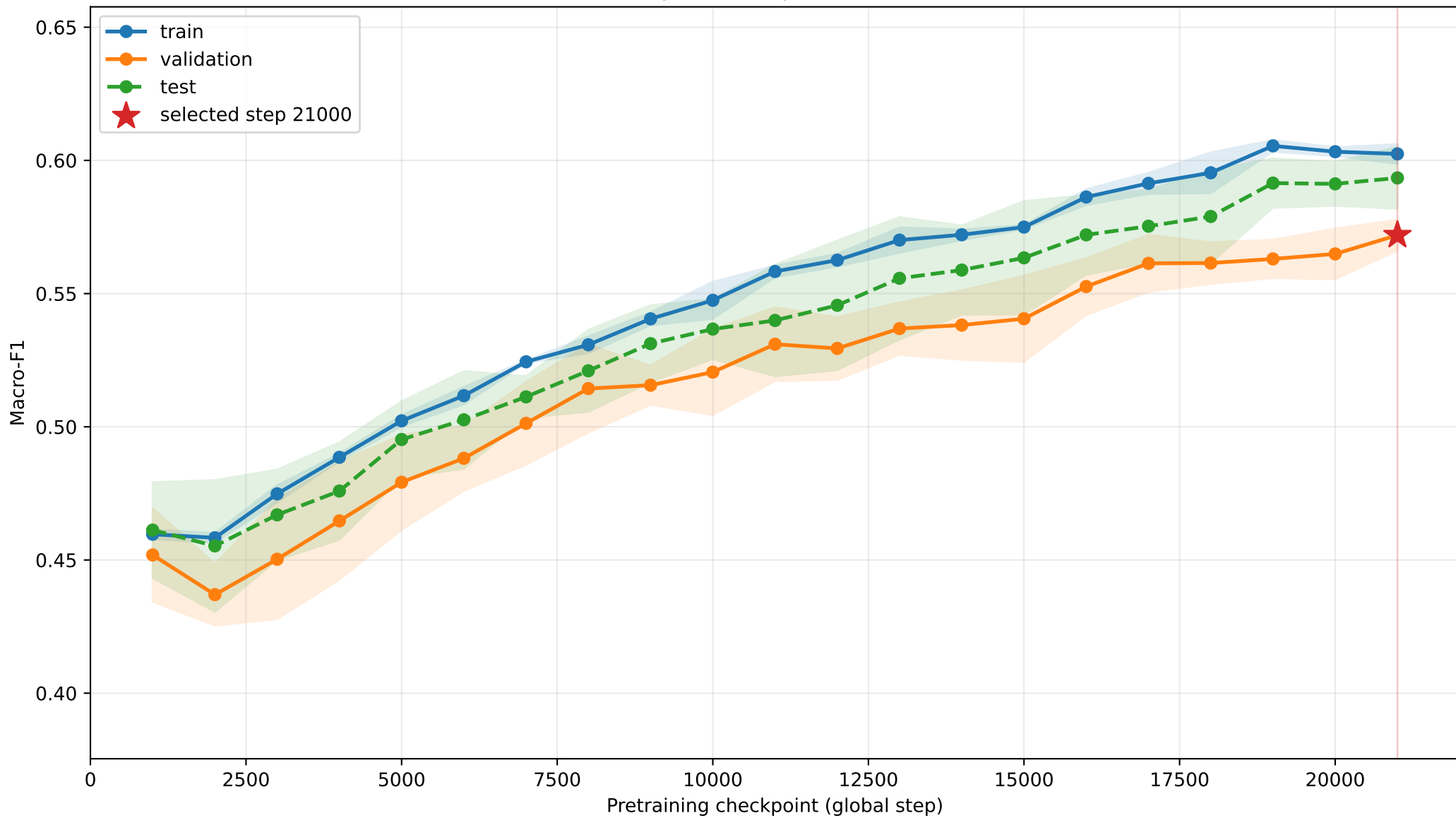
Galaxy10 linear probe: ViT-S/14
