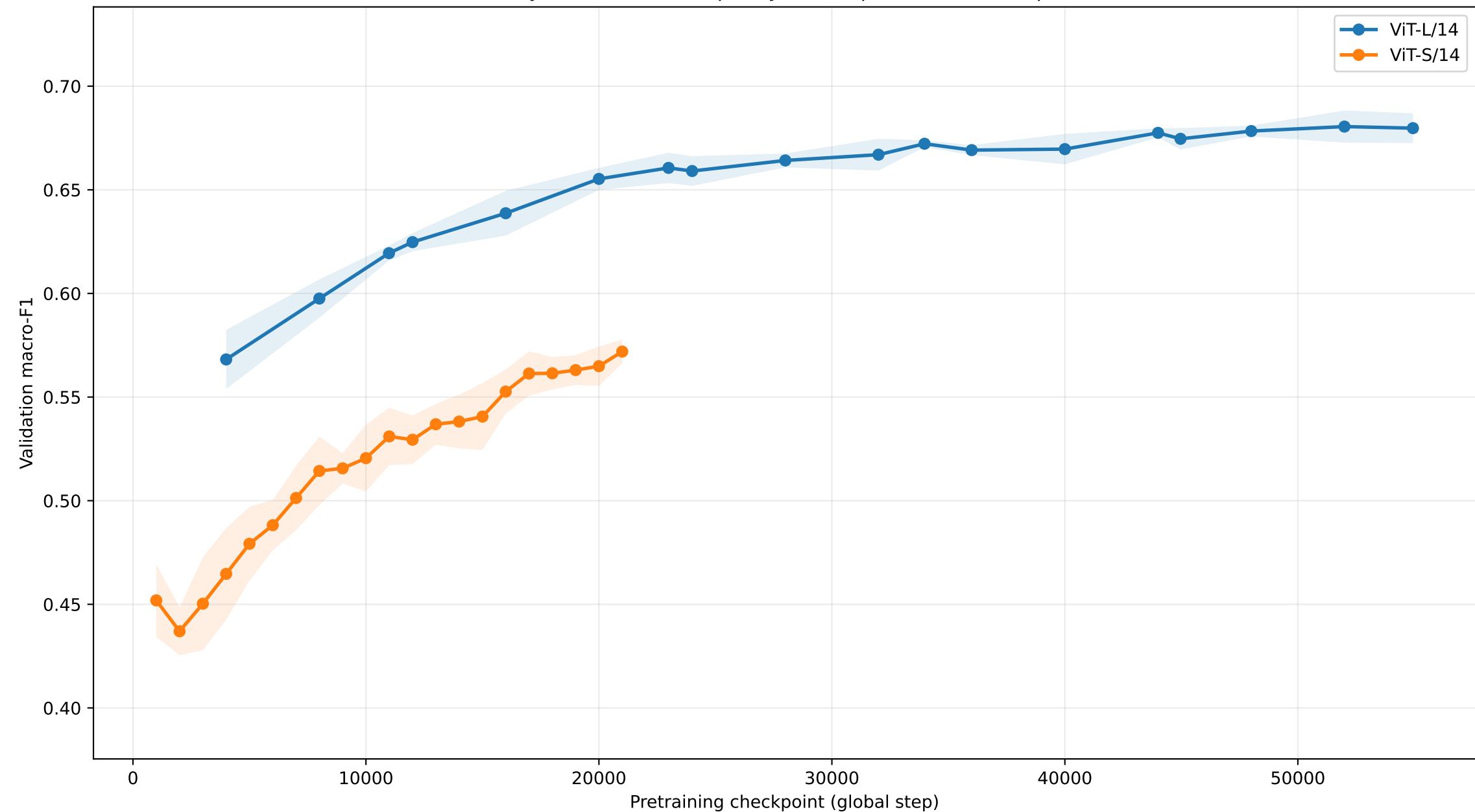
Galaxy10 downstream quality across pretrained checkpoints
