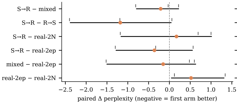
N = 1M: mean, 95% CI, per-seed ticks
