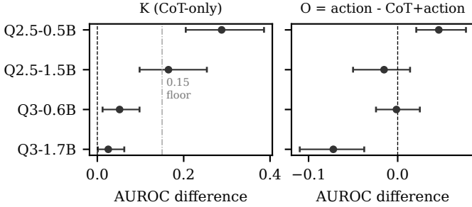
Fig. 2. Keyword reliance K (CoT-only) and narration override O with 95% skeleton-bootstrap CIs (Table V). Dash-dotted line: the pre-registered K floor of 0.15.
