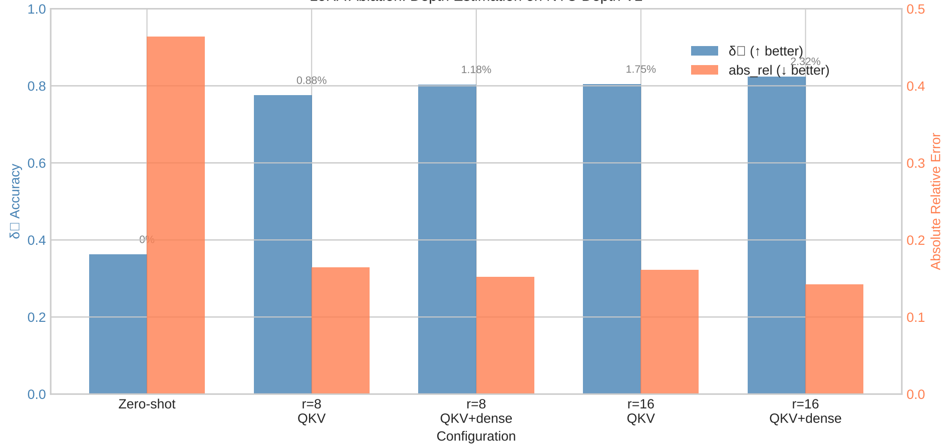
LoRA Ablation: Depth Estimation on NYU Depth V2
