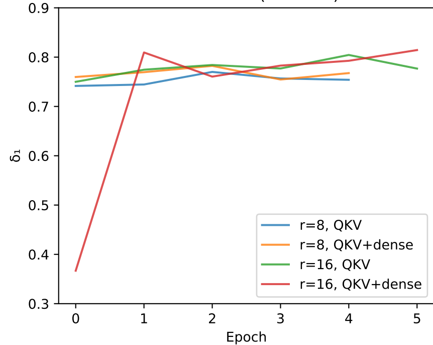
Validation \delta_1 ( \uparrow better)
