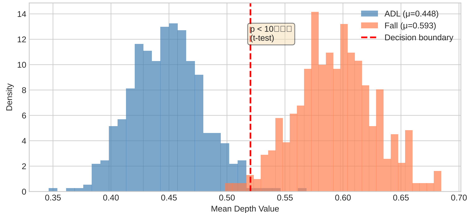
UR Fall Dataset Confound: Depth Distributions are Linearly Separable
