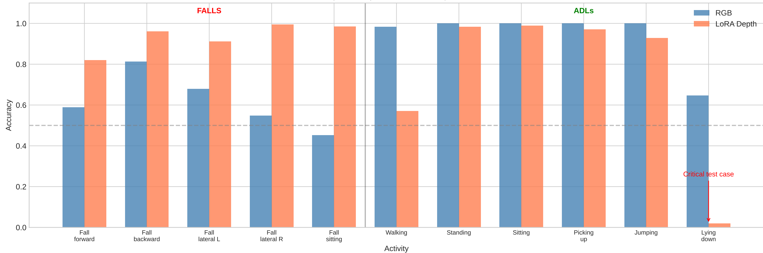
Per-Activity Accuracy: RGB vs LoRA Depth on UP-Fall
