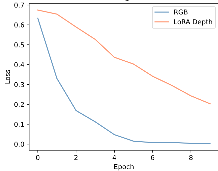
Training Loss
