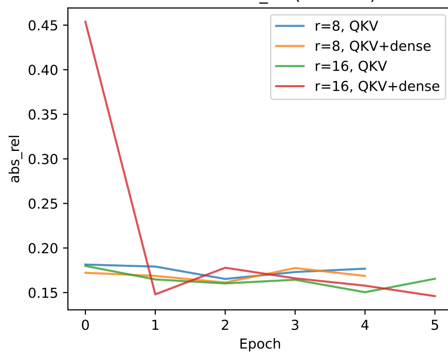
Validation abs_rel ( \downarrow better)
