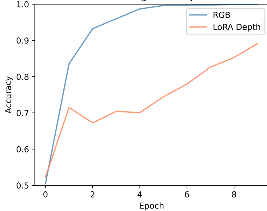
Training Accuracy
