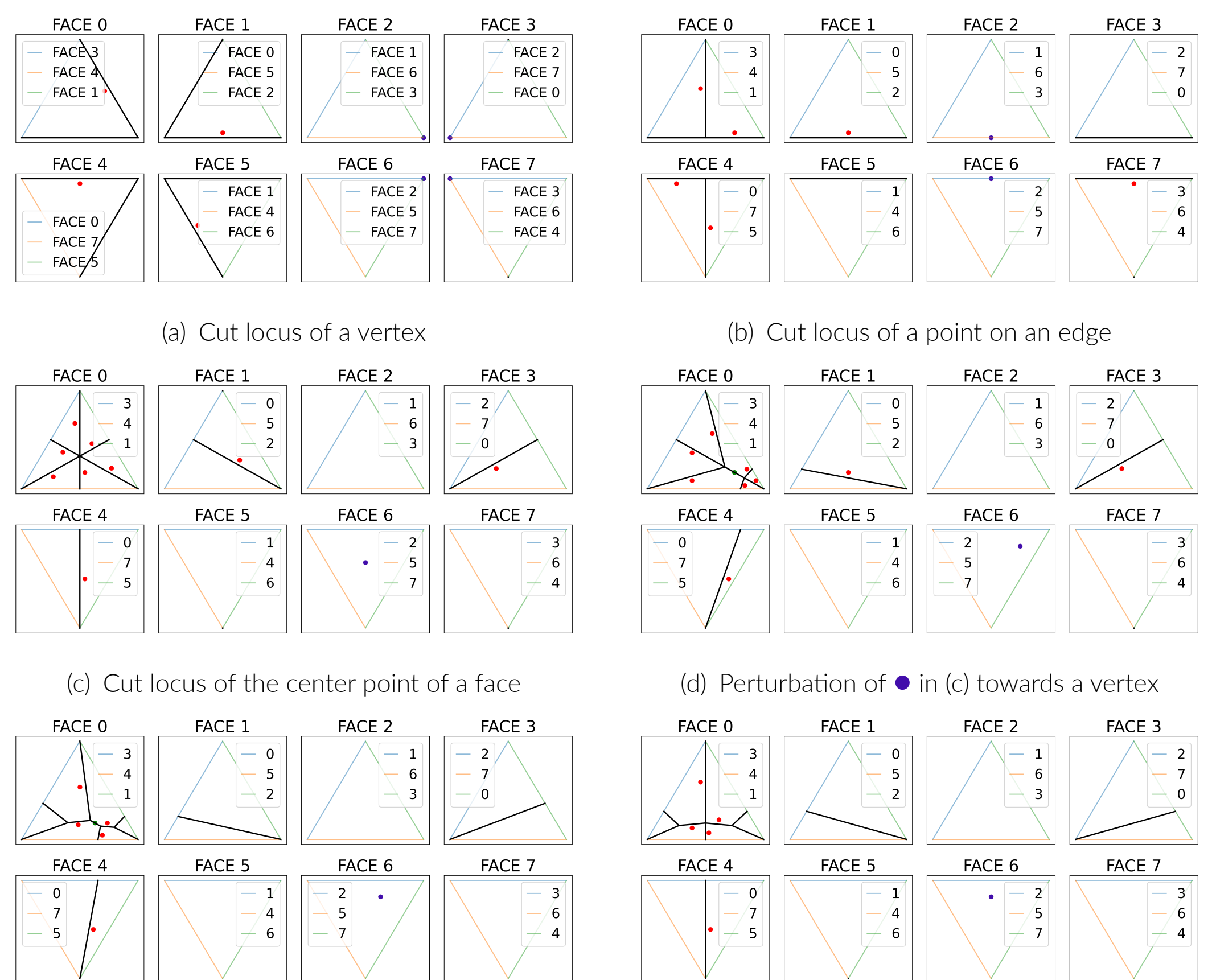
Figure 2. Construction of GMPR \sigma_2 . A path starting from \bullet approaches a cut locus line from the side indicated by \bullet . \bullet indicates free choice on which side to approach from. Observe that when a cut locus line has a unique endpoint on an octahedron vertex, \sigma_2 approaches the line from the 'right' side of that vertex (i.e. the first side encountered when moving counterclockwise around that vertex).
