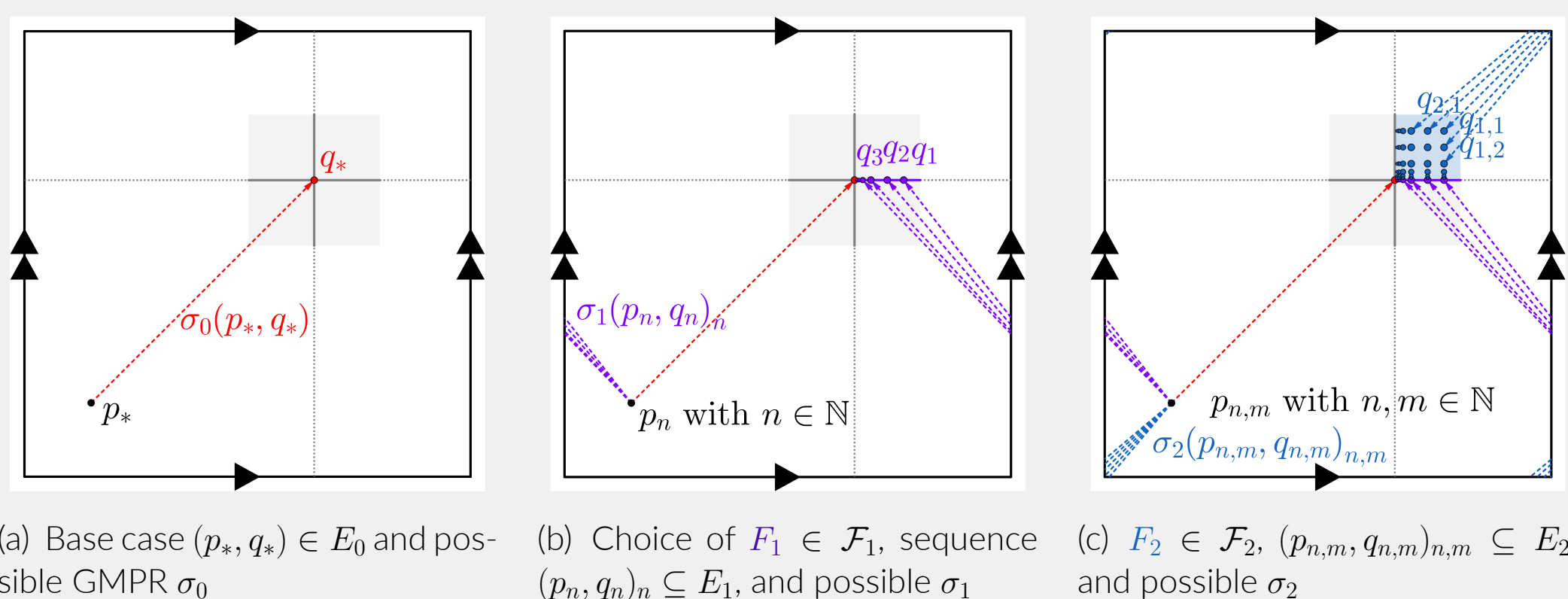
Figure 2. Mechanism of theorem when used on the 2-torus. Each embedding F \in \mathcal{F}_1 (resp. F' \in \mathcal{F}_2 ) embeds a simplex into \{p_*\} \times X by selecting the second factor to map to one of the shaded lines (resp. squares). F_1 (resp. F_2 ) is chosen to avoid \sigma_0(p_*, q_*) (resp. \sigma_1(p_n, q_n) ).
