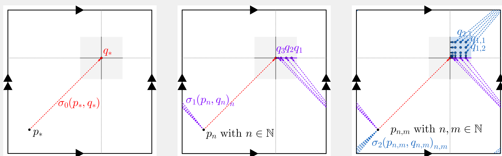
Figure 2. Mechanism of theorem when used on the 2-torus. Each embedding F \in \mathcal{F}_1 (resp. F' \in \mathcal{F}_2 ) embeds a simplex into \{p_*\} \times X by selecting the second factor to map to one of the shaded lines (resp. squares). F_1 (resp. F_2 ) is chosen to avoid \sigma_0(p_*, q_*) (resp. \sigma_1(p_n, q_n)_n ).
