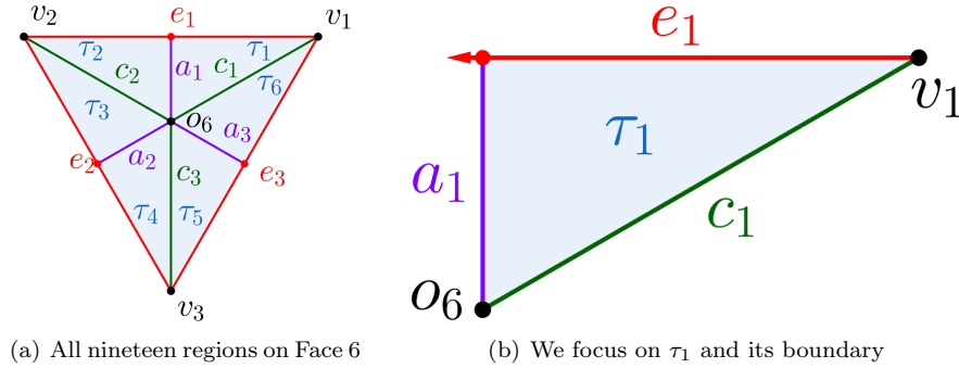
Figure 11: Partition of Face 6 into regions with isometric cut loci
