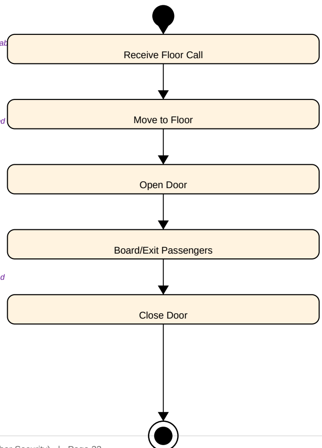
Activity Diagram
