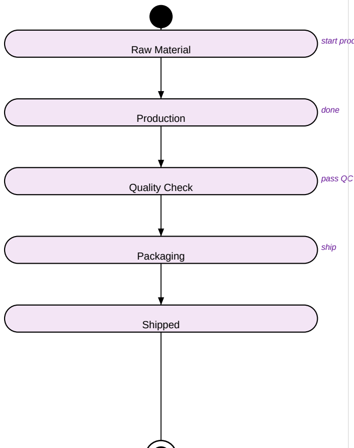
Statechart Diagram
