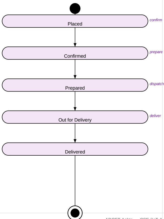
Statechart Diagram
