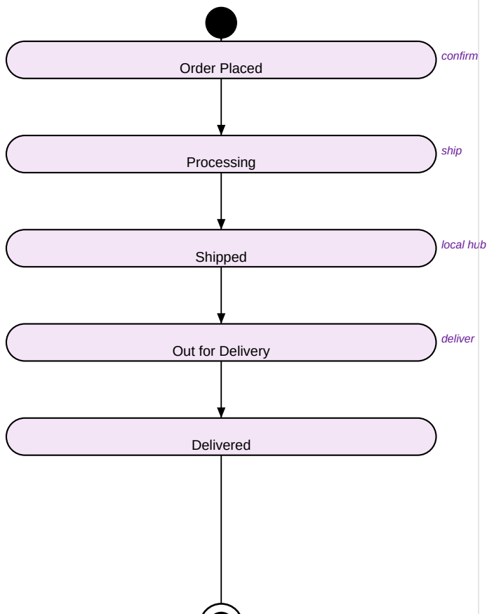
Statechart Diagram
