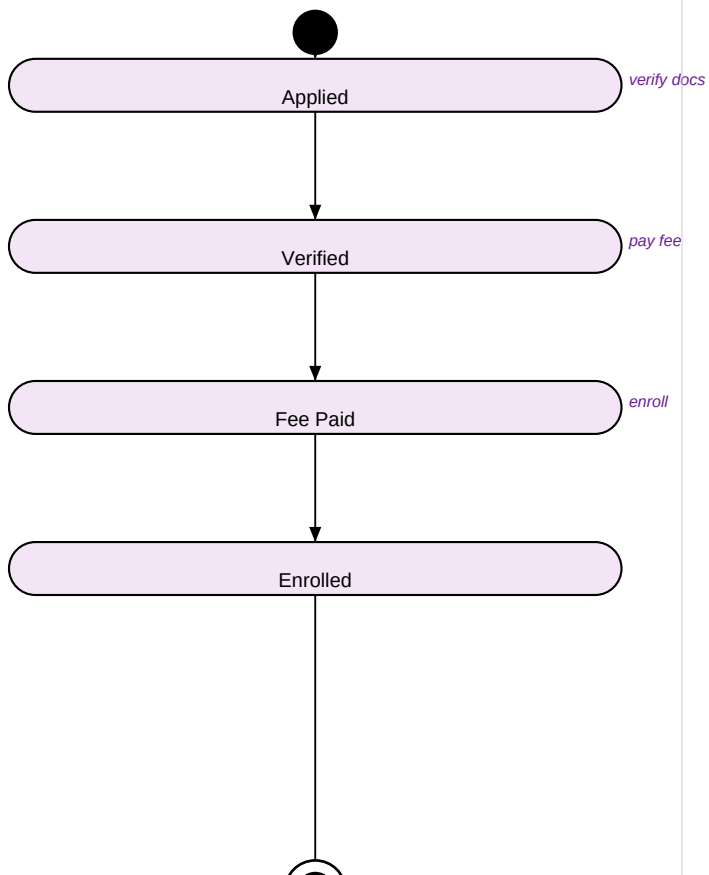
Statechart Diagram
