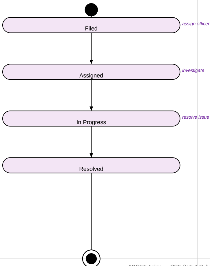
Statechart Diagram
