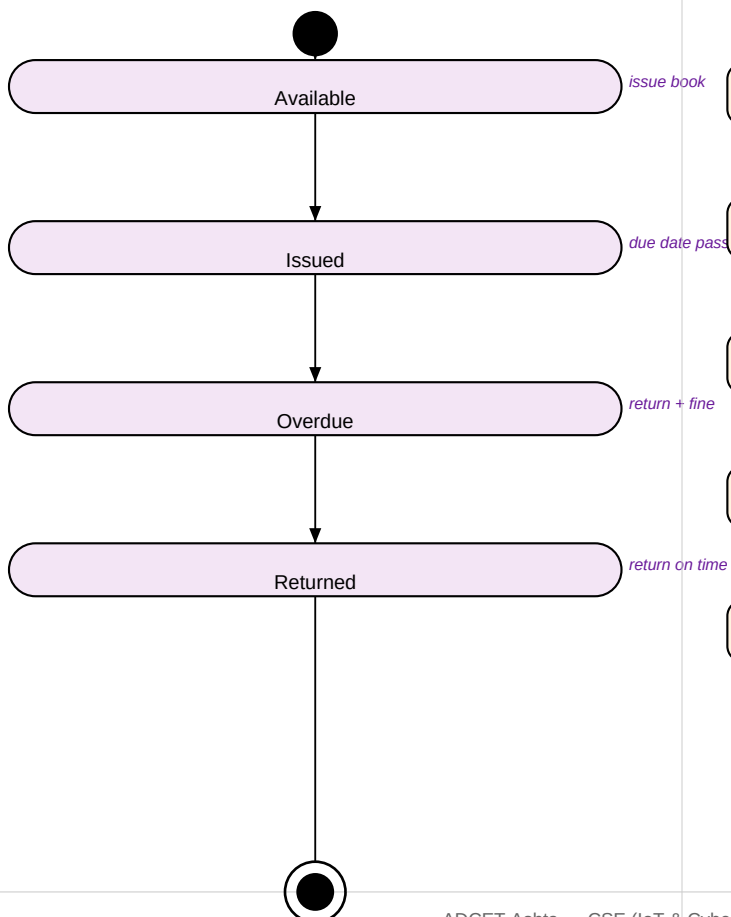
Statechart Diagram
