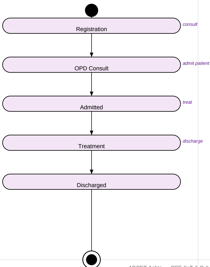
Statechart Diagram
