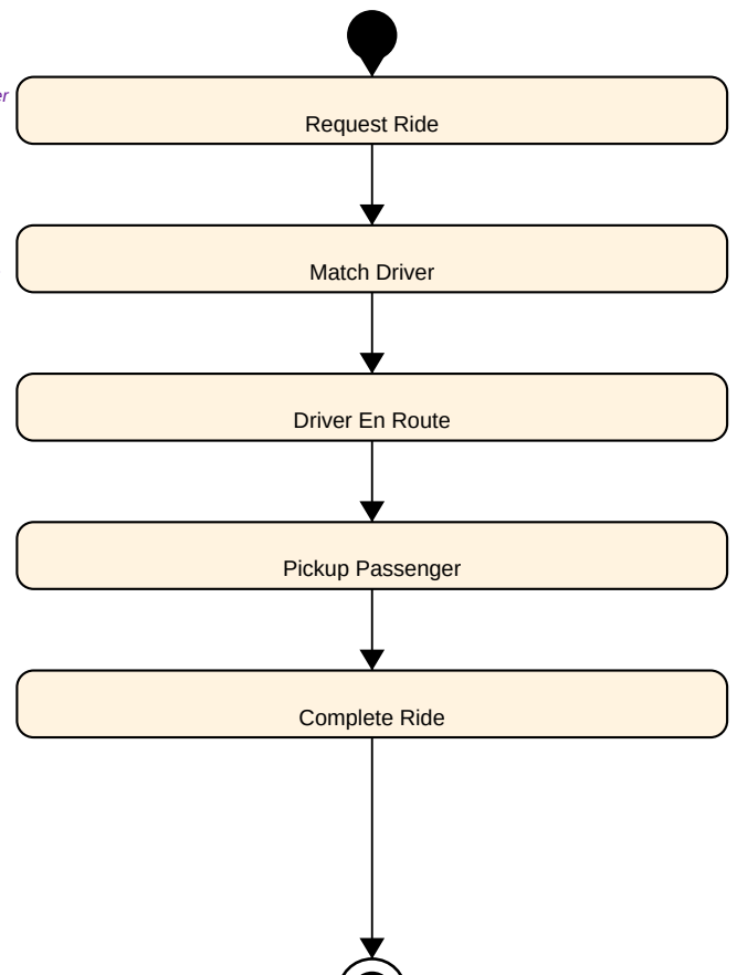
Activity Diagram
