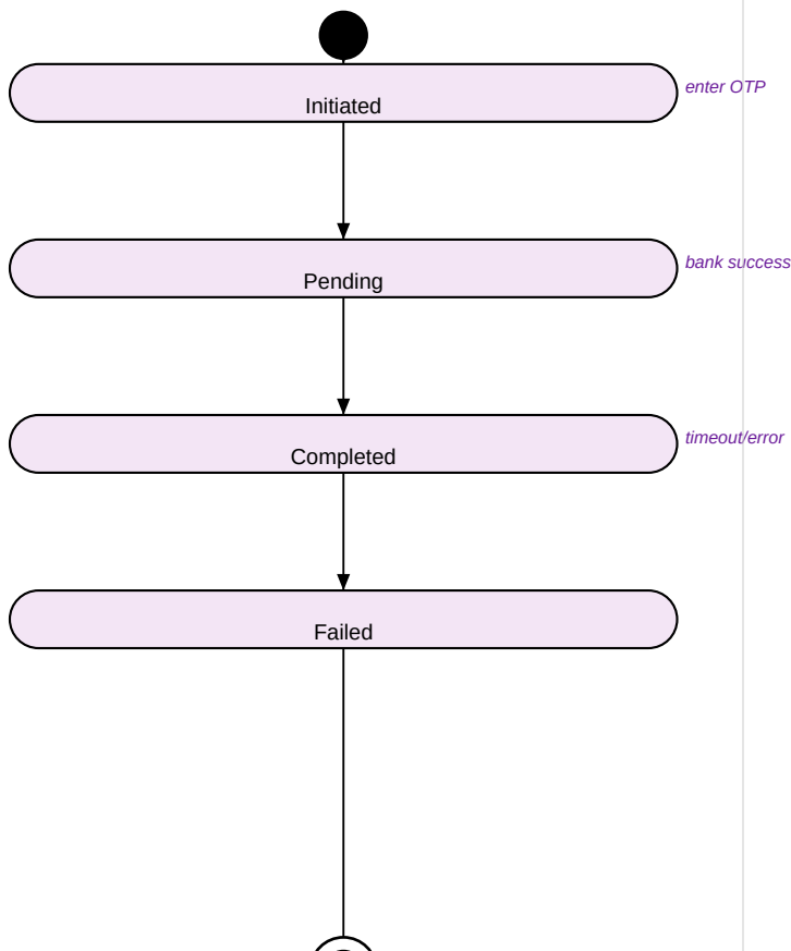
Statechart Diagram
