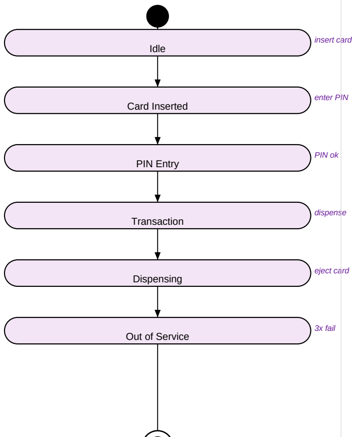
Statechart Diagram
