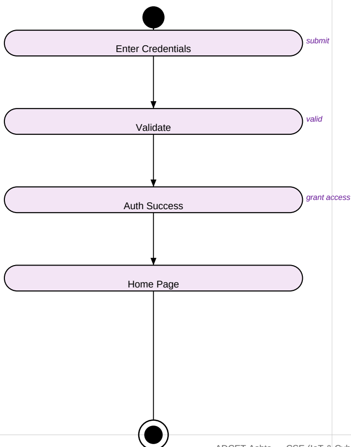
Statechart Diagram
