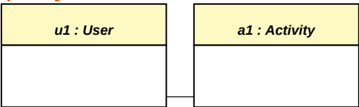
Object Diagram:
