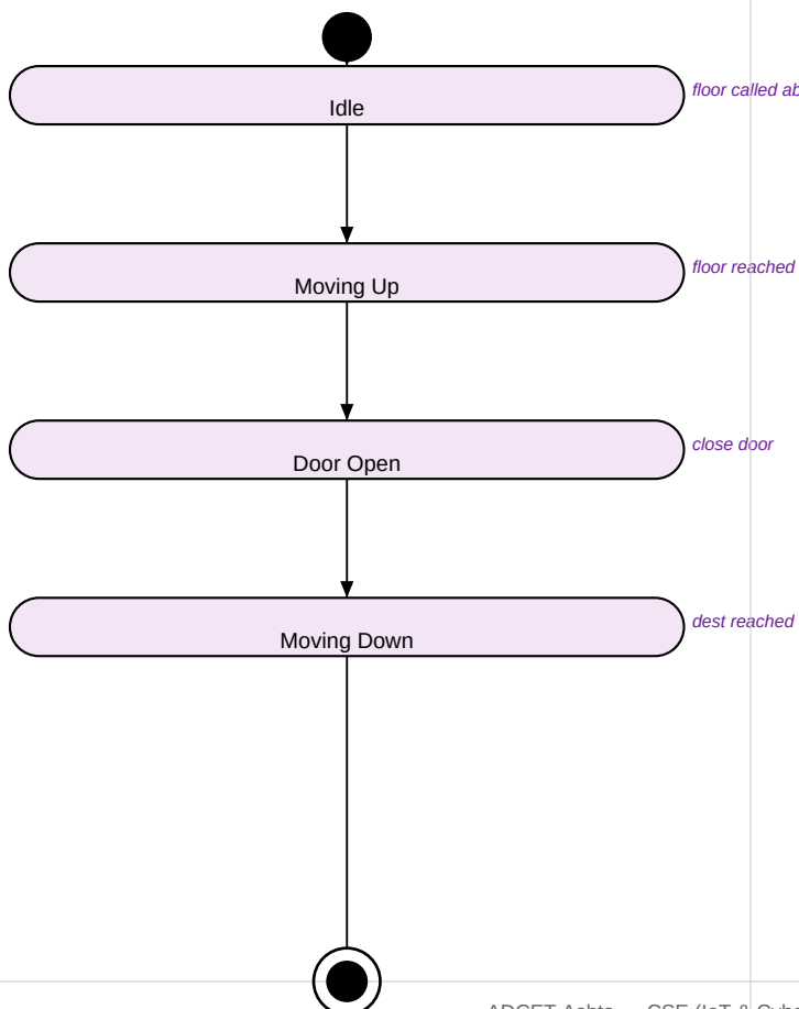
Statechart Diagram
