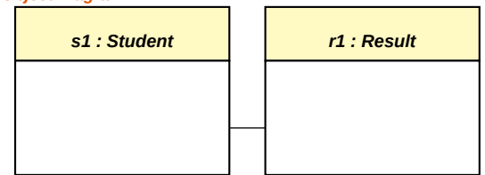
Object Diagram:
