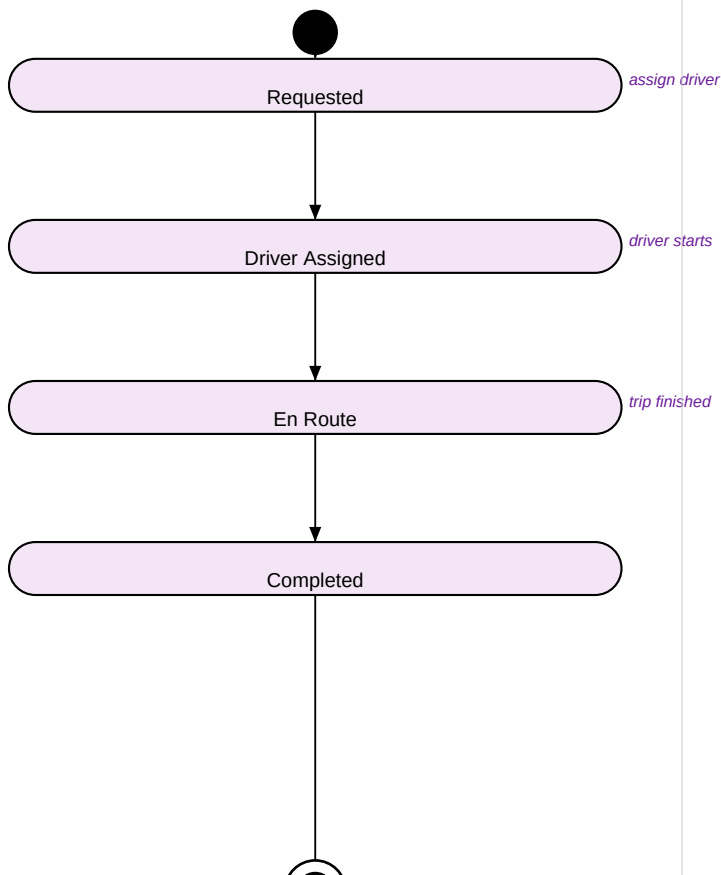
Statechart Diagram
