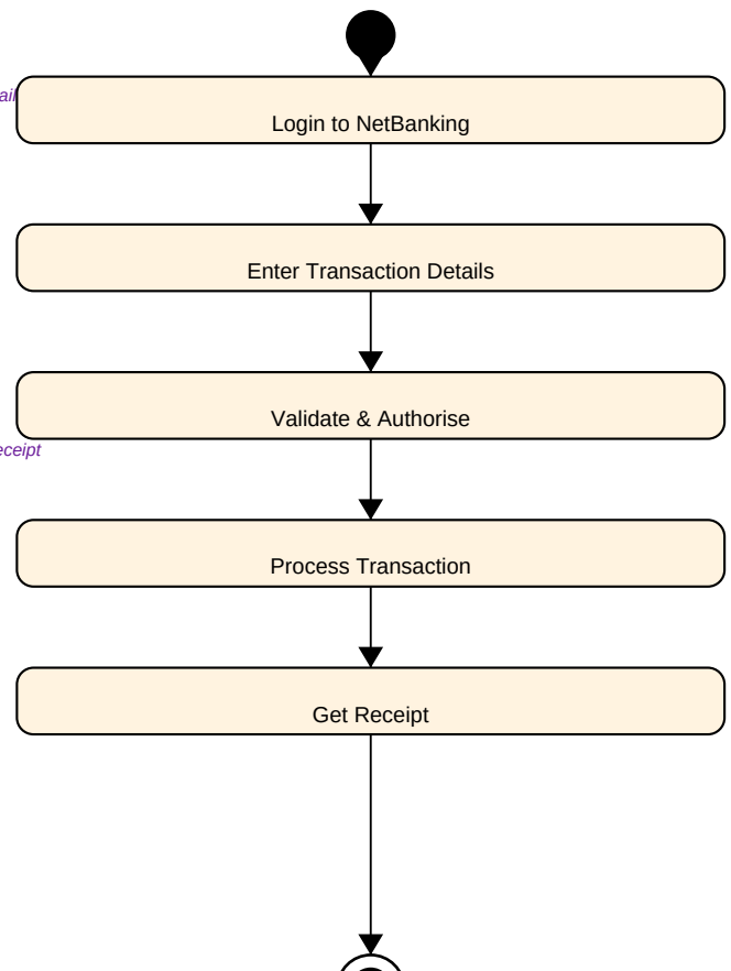
Activity Diagram
