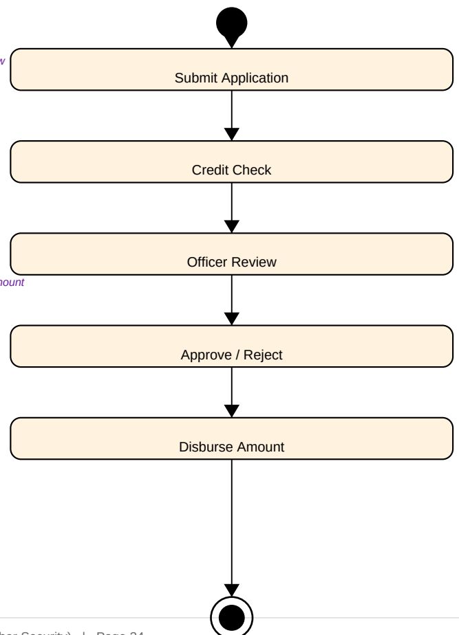
Activity Diagram
