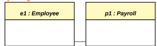
Object Diagram:
