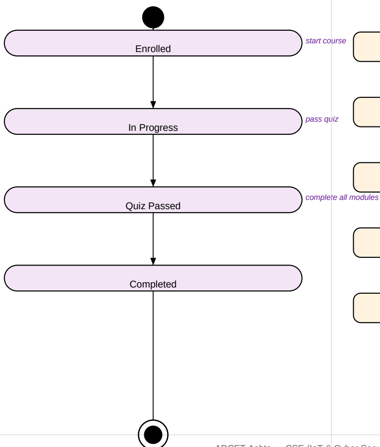
Statechart Diagram
