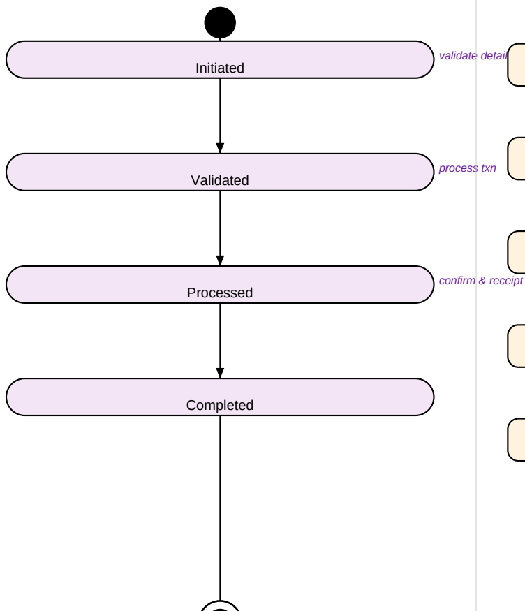
Statechart Diagram
