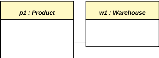
Object Diagram:
