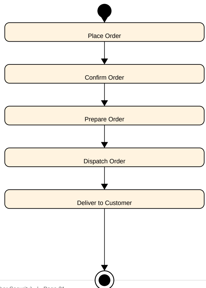
Activity Diagram
