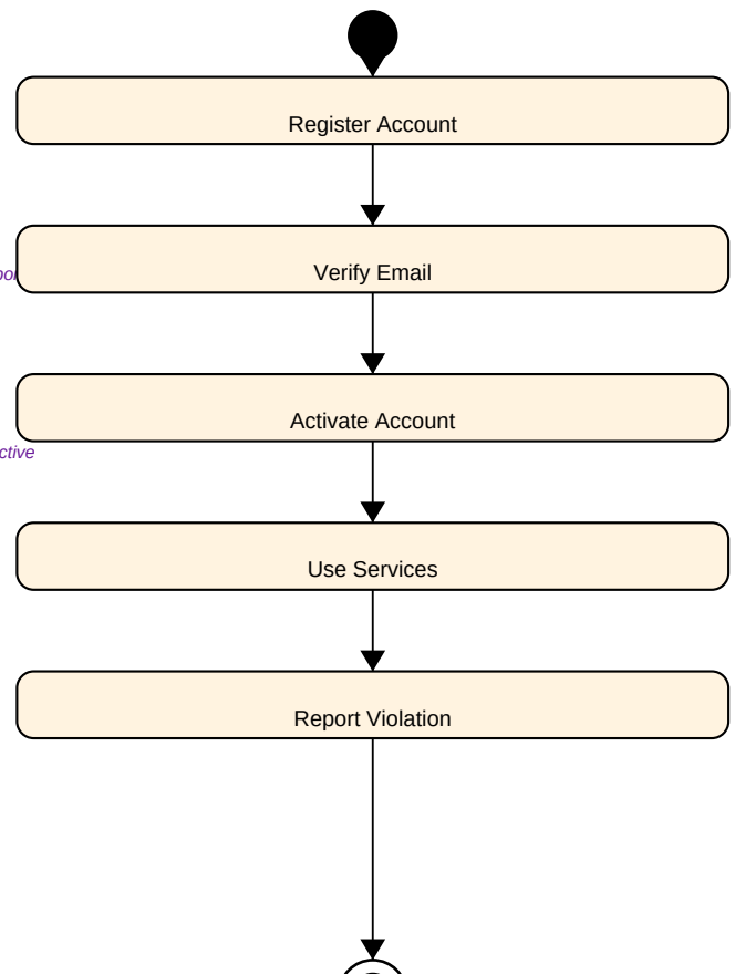
Activity Diagram
