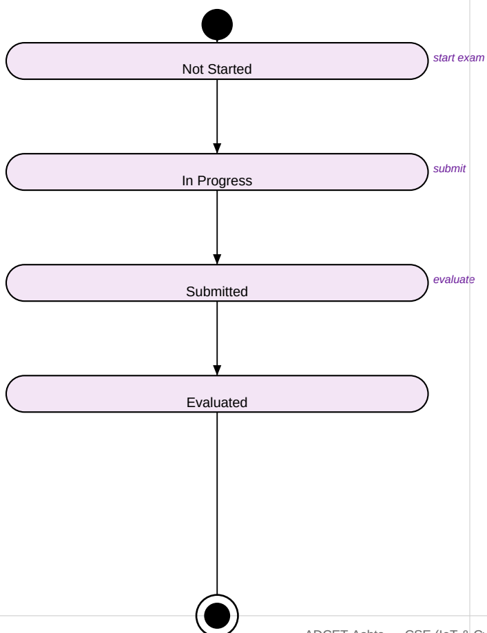
Statechart Diagram
