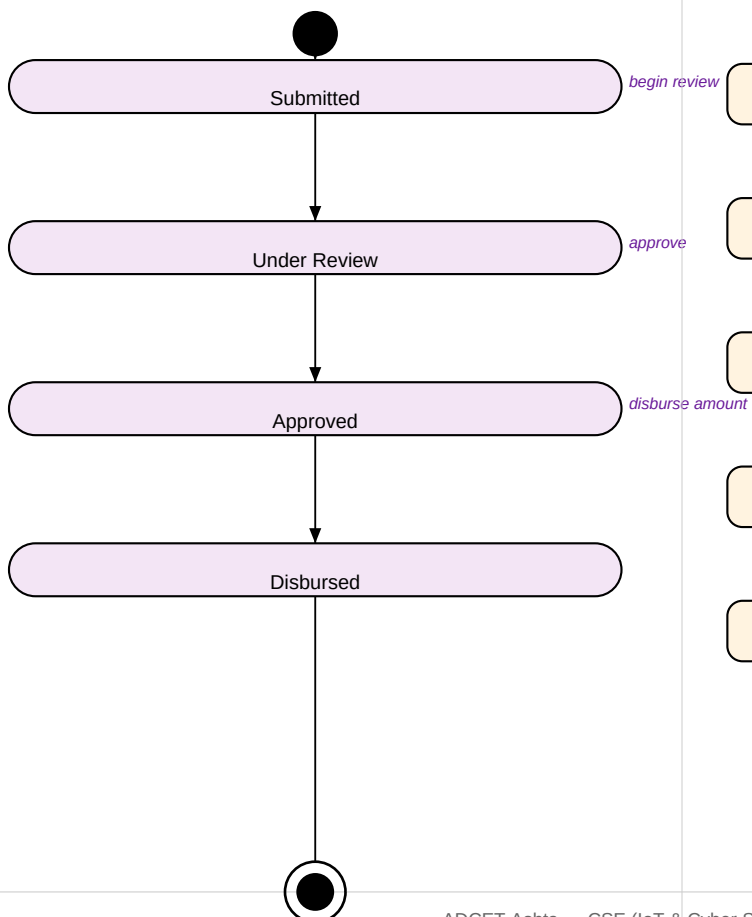
Statechart Diagram
