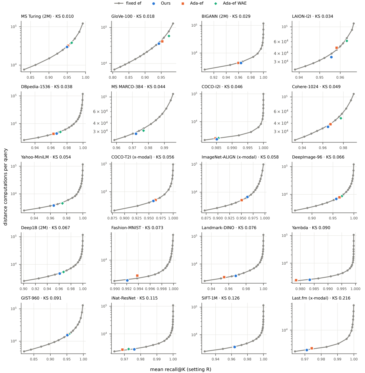
Figure 3: Distance computations per query against mean recall, setting R. Grey: HNSW with fixed ef . Points below the curve reach the same recall with less work. Panels are ordered by KS, from near-Gaussian (top left) to non-Gaussian (bottom right).
