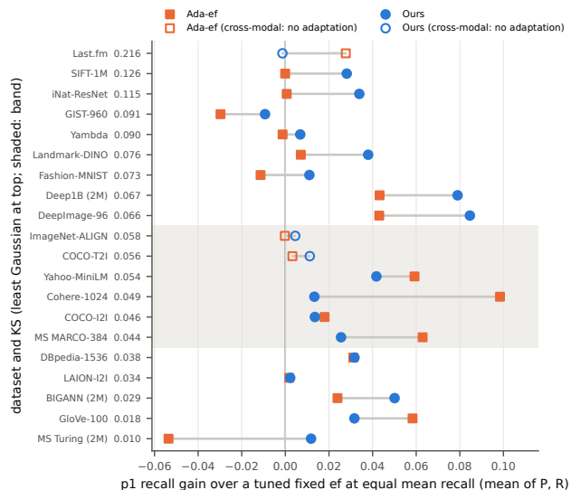
Figure 1: Tail recall gained over a fixed ef at the same mean recall, for Ada-ef and for our empirical score, on 20 datasets ordered by how far they are from Gaussian (KS, higher is less Gaussian). Above the shaded band, where Ada-ef’s Gaussian model does not hold, the empirical score wins on every dataset whose queries come from the same modality as the database. Below it, on near-Gaussian text embeddings, Ada-ef usually wins. Hollow markers: cross-modal queries, where neither score adapts.
