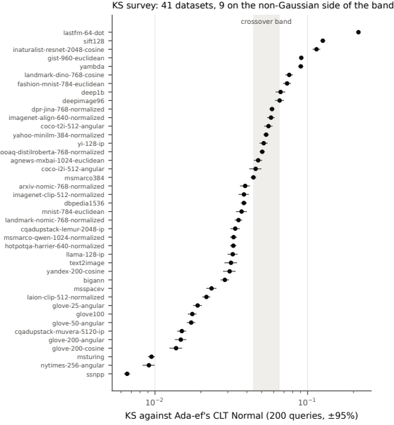
Figure 2: KS between each query’s similarities and Ada-ef’s Gaussian, mean over 200 queries with 95% interval, for 41 public datasets. Shaded: the band in which neither score ranks queries clearly better. GloVe-200 appears twice, from ann-benchmarks and from VIBE.
