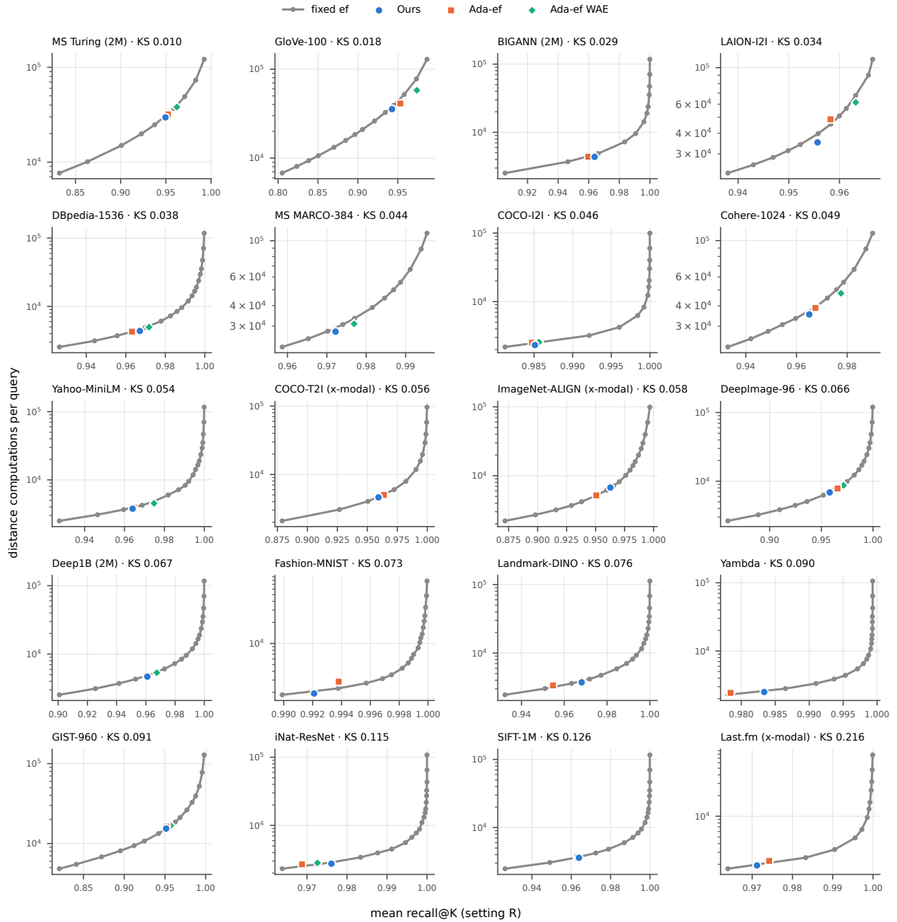
Figure 3: Distance computations per query against mean recall, setting R. Grey: HNSW with fixed ef . Points below the curve reach the same recall with less work. Panels are ordered by KS, from near-Gaussian (top left) to non-Gaussian (bottom right).
