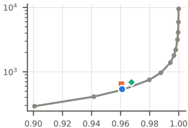
Deep1B (2M) · KS 0.067
