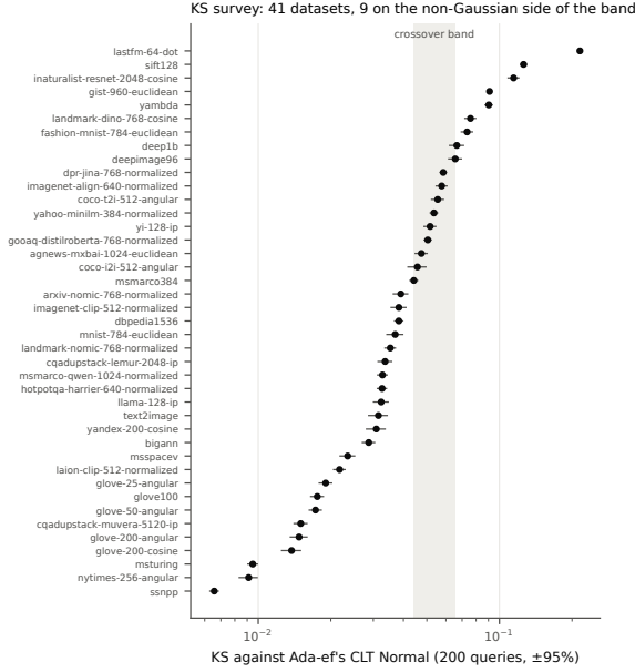
Figure 2: KS between each query’s similarities and Ada-ef’s Gaussian, mean over 200 queries with 95% interval, for 41 public datasets. Shaded: the band in which neither score ranks queries clearly better. GloVe-200 appears twice, from ann-benchmarks and from VIBE.
