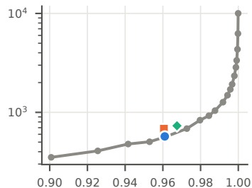
Deep1B (2M) · KS 0.067
