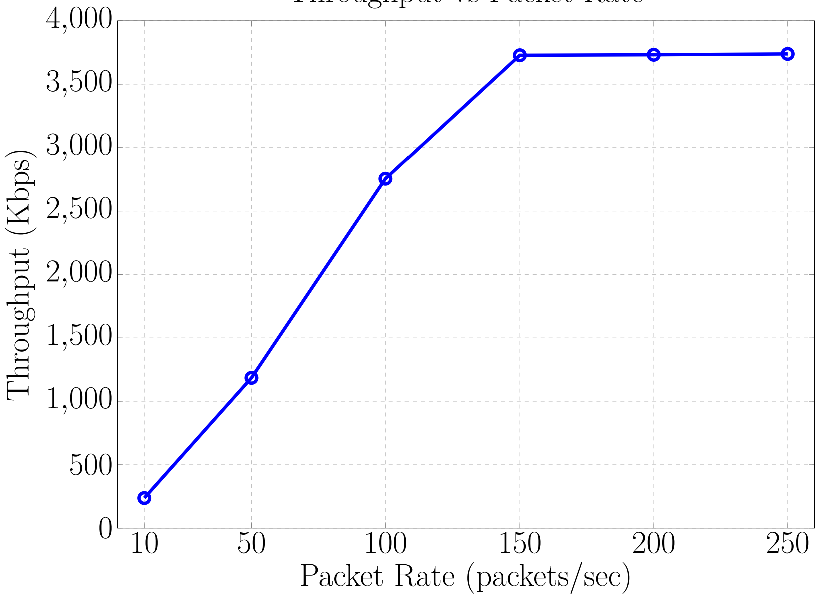
Throughput vs Packet Rate
