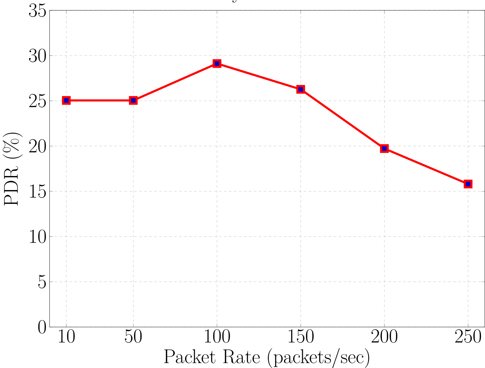
Packet Delivery Ratio vs Packet Rate
