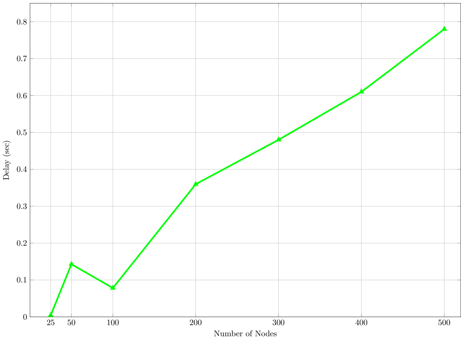
Delay vs Number of Nodes
