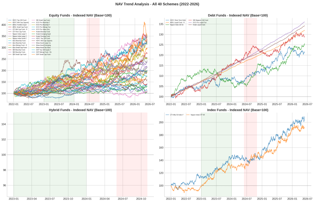
Figure 1: Indexed NAV trends - 40 funds. Green=2023 bull run, red=2024 correction.
