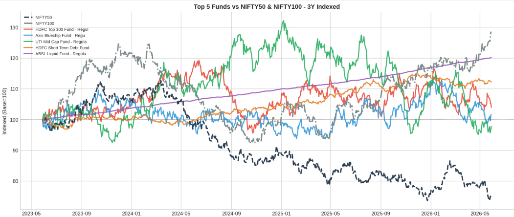
Figure 6: Top 5 funds vs NIFTY50 & NIFTY100. 3-year indexed. TE=Tracking Error vs NIFTY100.
