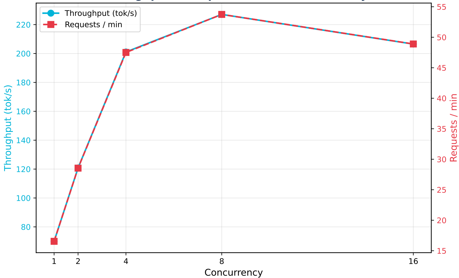
Throughput & Request Rate vs Concurrency
