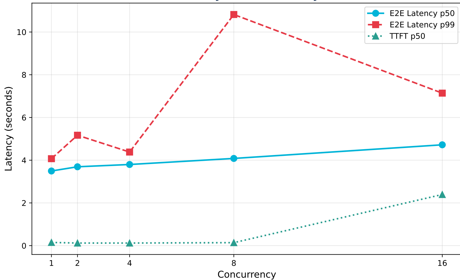
Latency vs Concurrency
