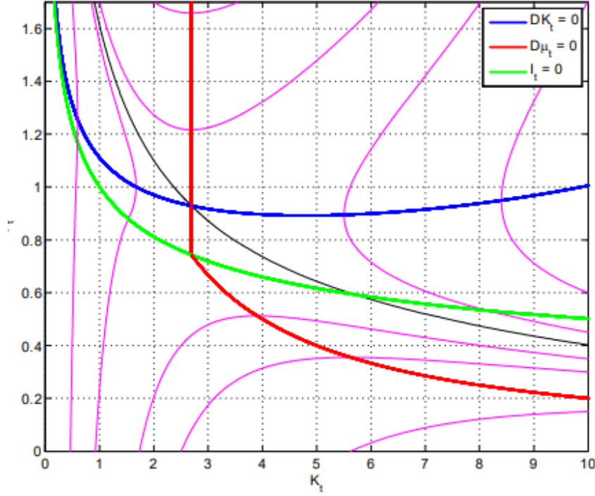
Figure 2: The phase diagram for (K_t, p_t) with irreversible investment.
