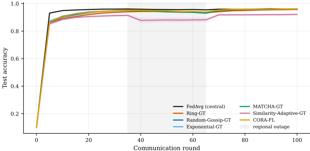
Digits, domain-correlated non-IID outage
