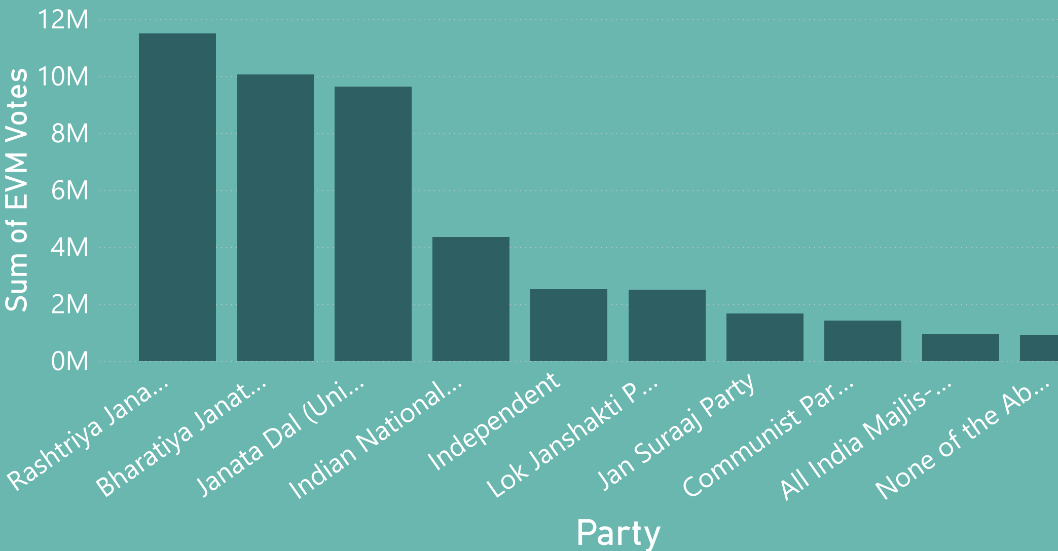
EVM Votes by Party
