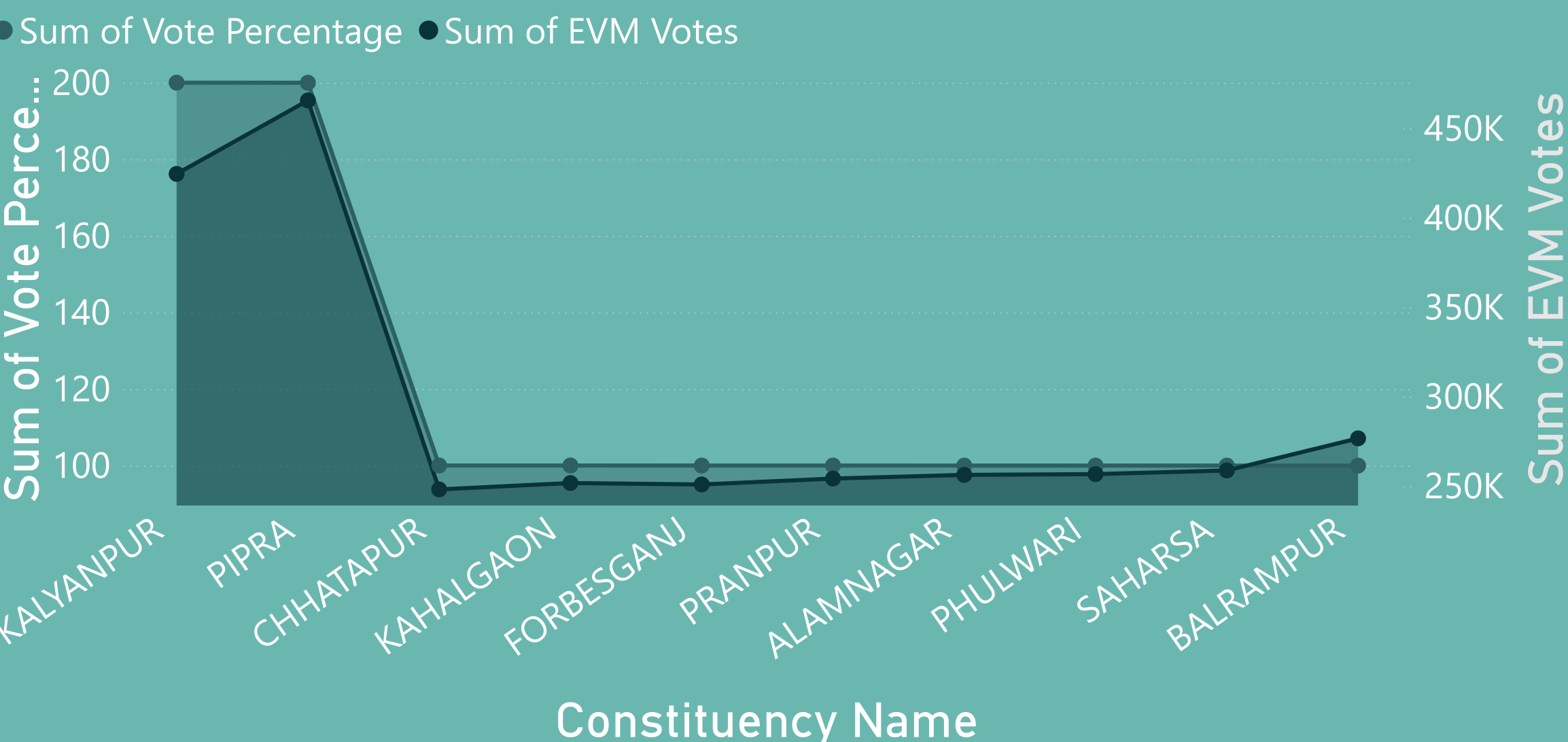
Vote Percentage and EVM Votes by Constituency Name
