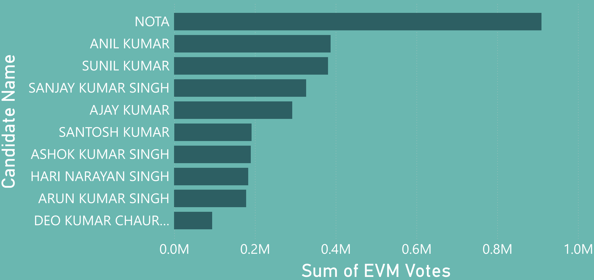
EVM Votes by Candidate Name
