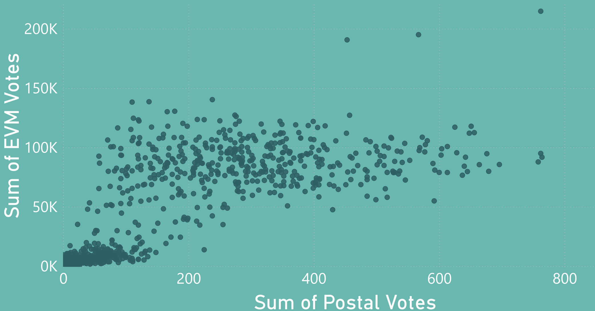
Postal Votes and EVM Votes by Total Votes
