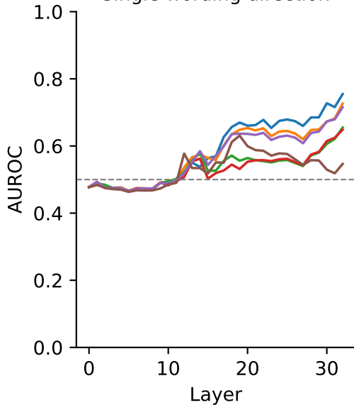
Single wording direction
