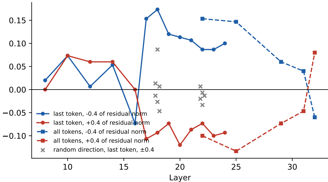
Change in accuracy, negated items
