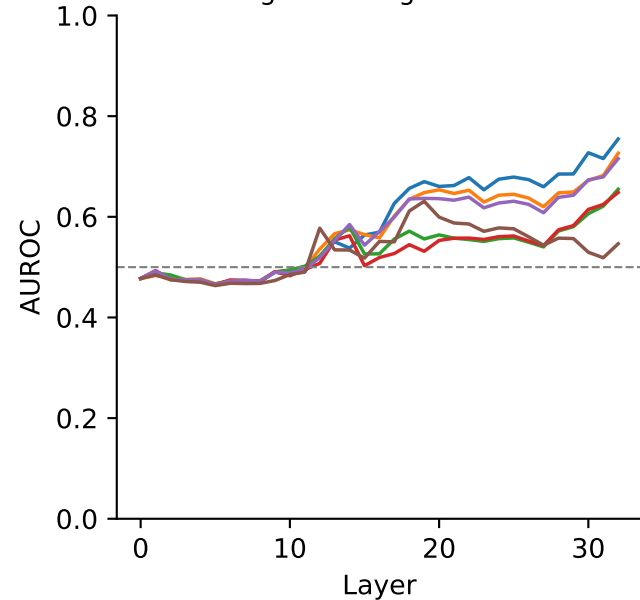
Single wording direction
