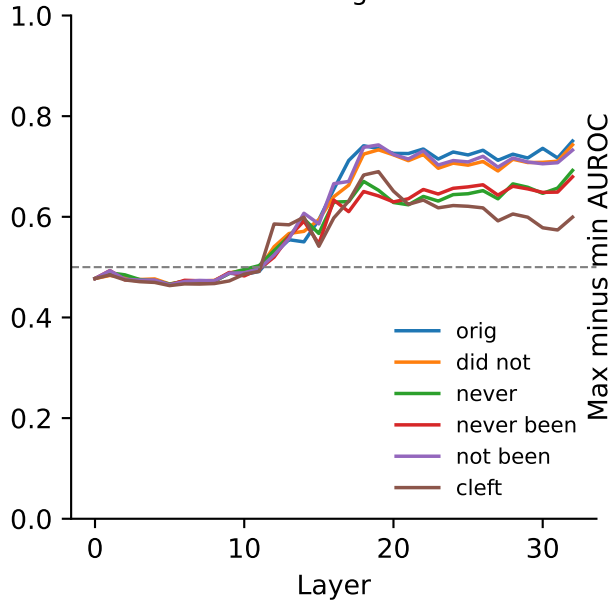
Mixed wording direction
