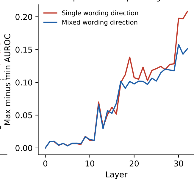
Spread across phrasings
