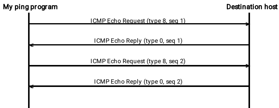
Fig 2: Working of the ping program
