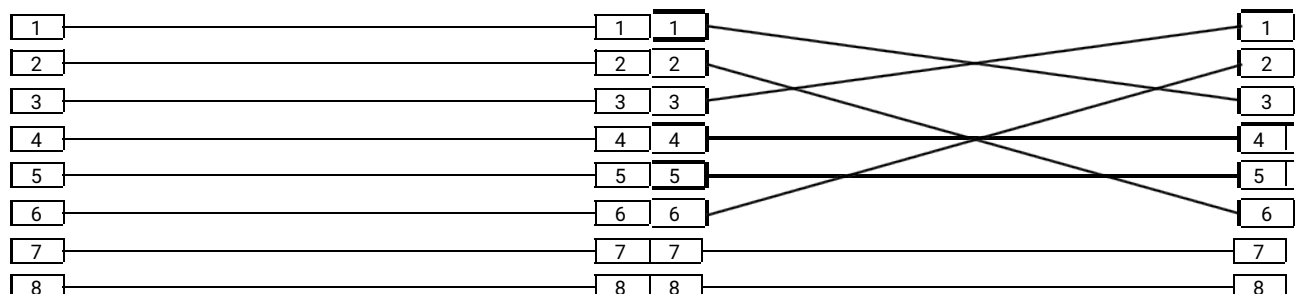
Fig 1: Straight-through cable (pin 1 to 1, 2 to 2 ...) Fig 2: Crossover cable (1 to 3, 2 to 6, 3 to 1, 6 to 2)
