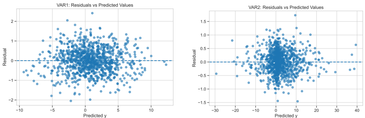
Figure 5: Residuals against predicted values on the training data: VAR1 (left), VAR2 (right).
