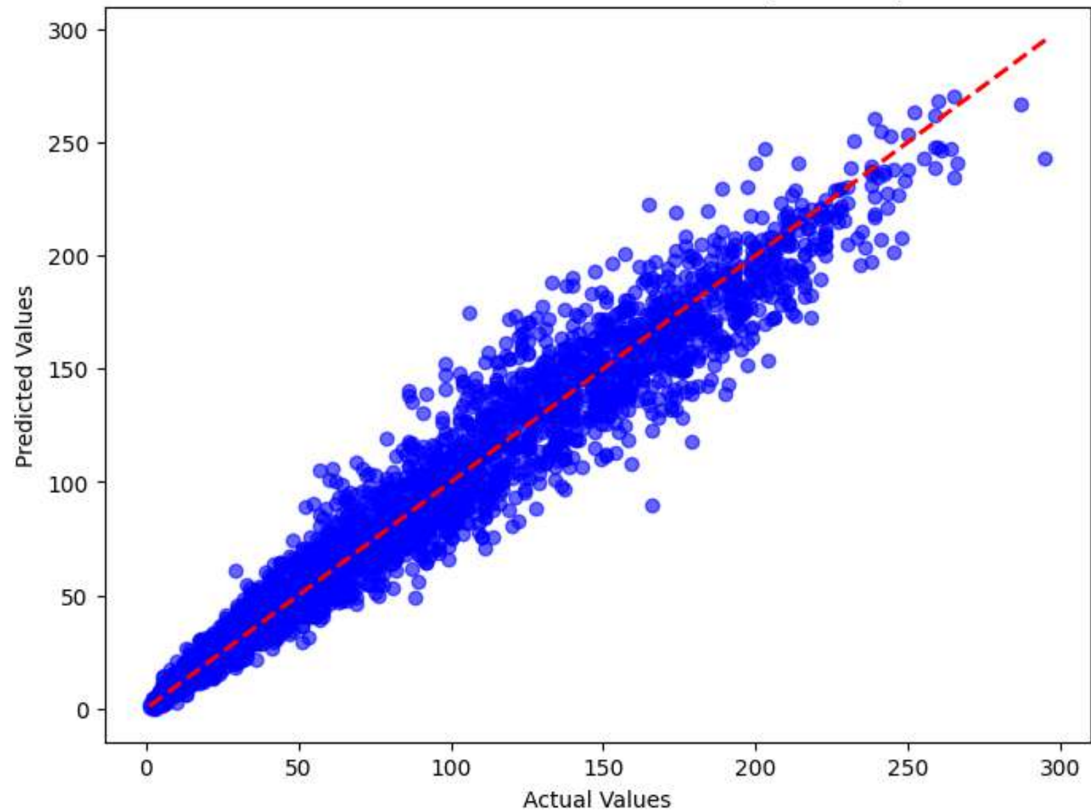
Actual vs Predicted Calories Burned (CatBoost)
