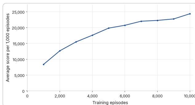
Figure 2. Average score per 1,000 training episodes. Self-play score rises from 8,384 to 24,382.
