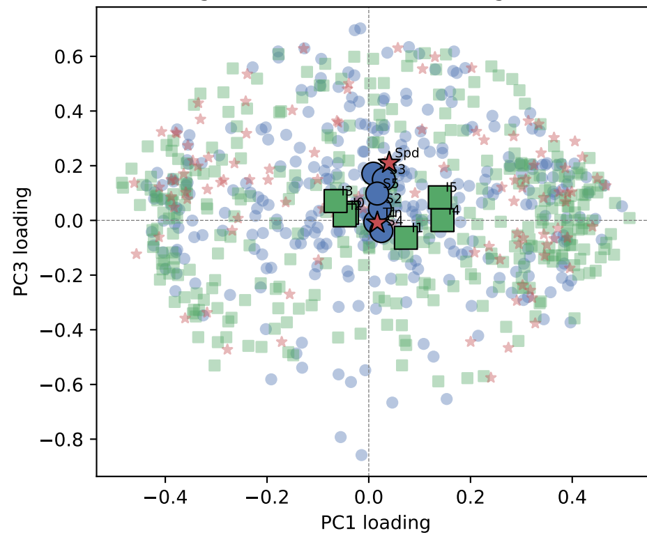
Neuronal embeddings — PC1 vs PC3 (54 agents, dots=individual, large=mean)
