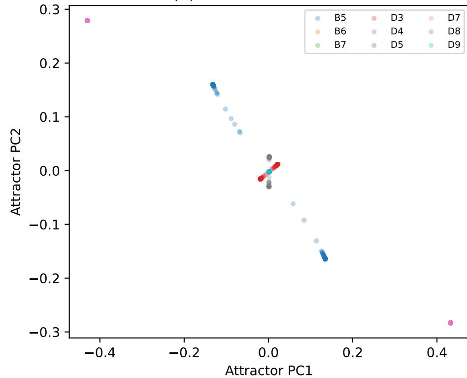
D4: Attractor fingerprints in 2D (1 rep per mouse, 200 inits each)
