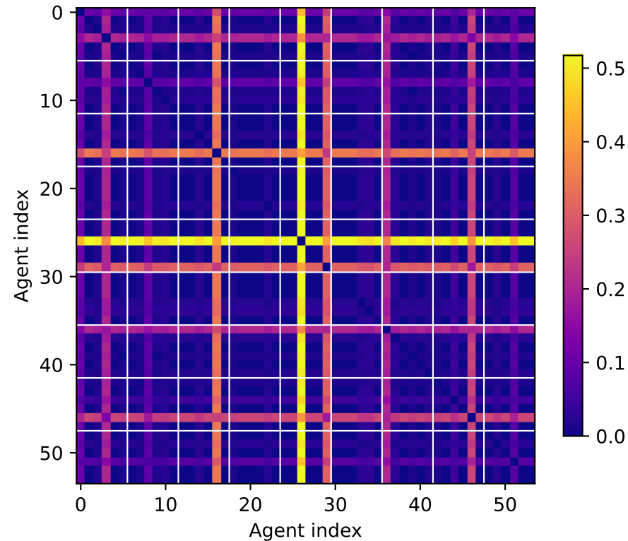
D4: 54×54 attractor landscape distances (sliced Wasserstein)
