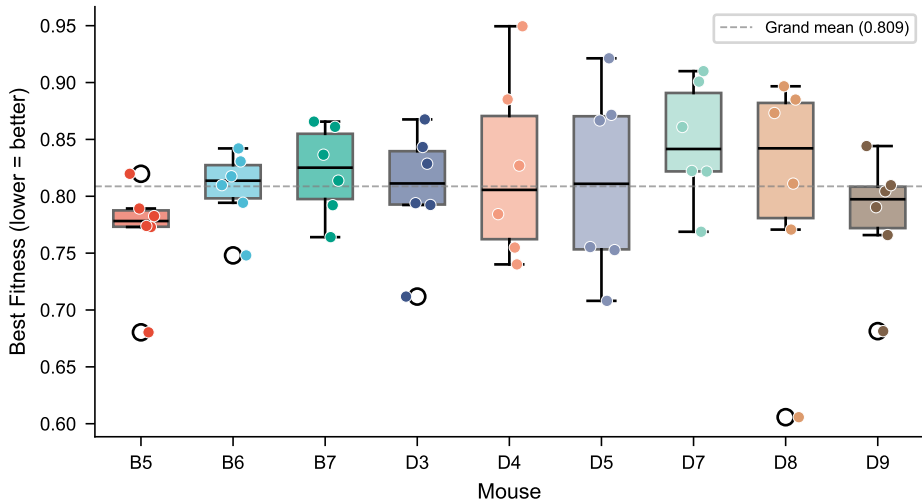
Fitness Convergence by Mouse
