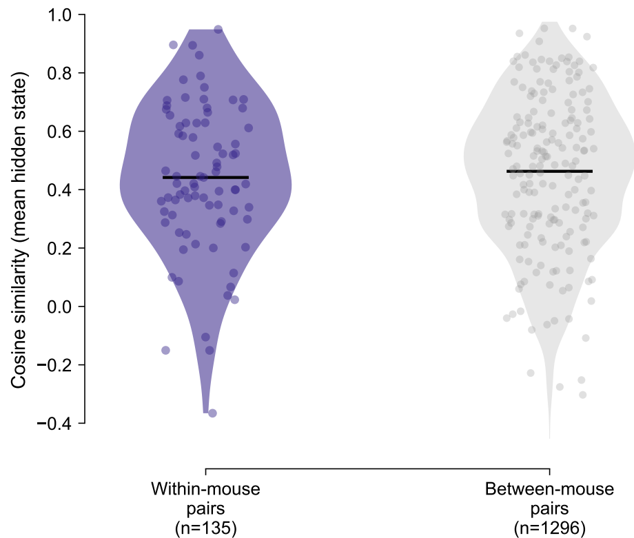
B Trajectory RSM: within vs between mouse (Mann-Whitney p = 0.509 ; n.s.)
