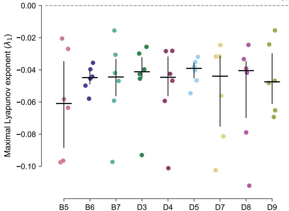
A Per-mouse \lambda_1 (all agents: \lambda_1 < 0 , ANOVA p = 0.943 ) \lambda_1 = 0 (stability boundary)
