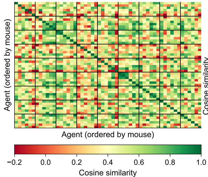
B Representational Similarity Matrix
