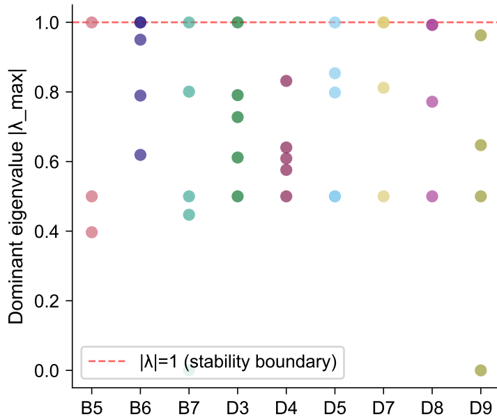
B Spectral radius at fixed points ANOVA F=0.99 , p=0.460
