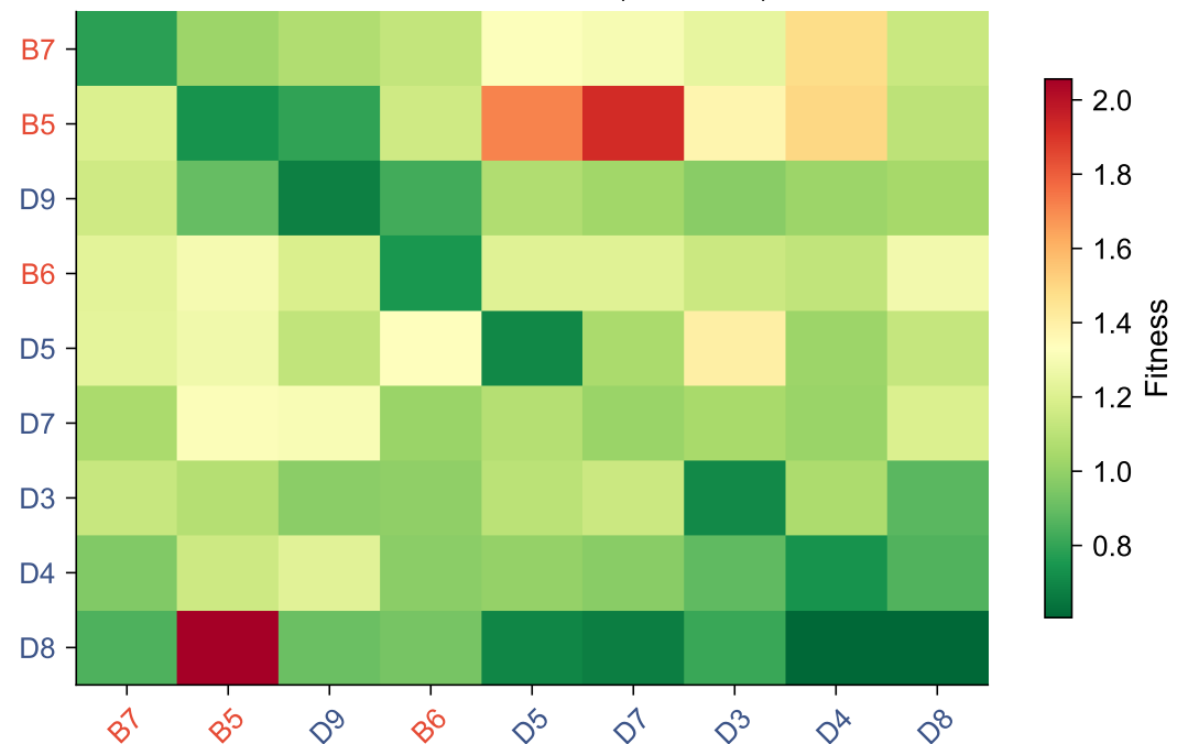
Generalization Matrix (clustered)
