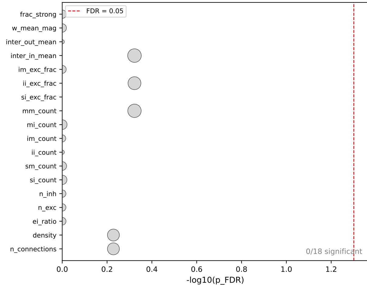
Evolved agents (9 mice x 6 replicates)
