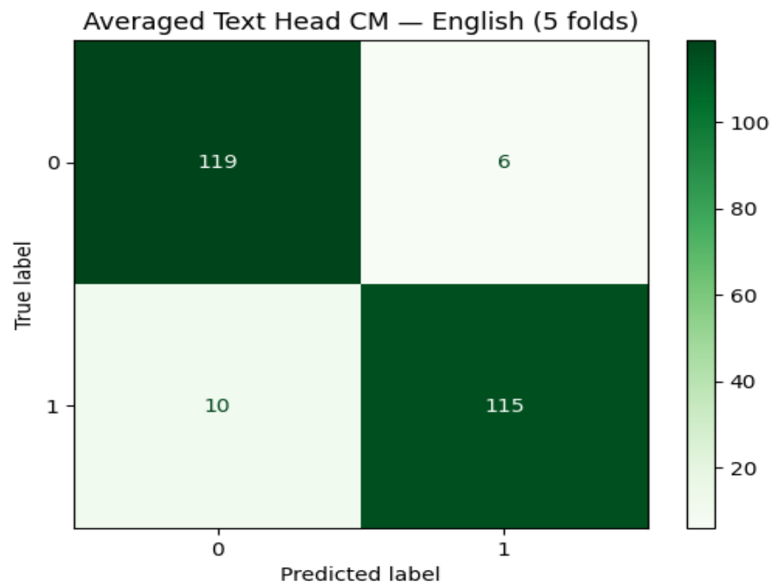
Averaged Text Head CM — English (5 folds)
