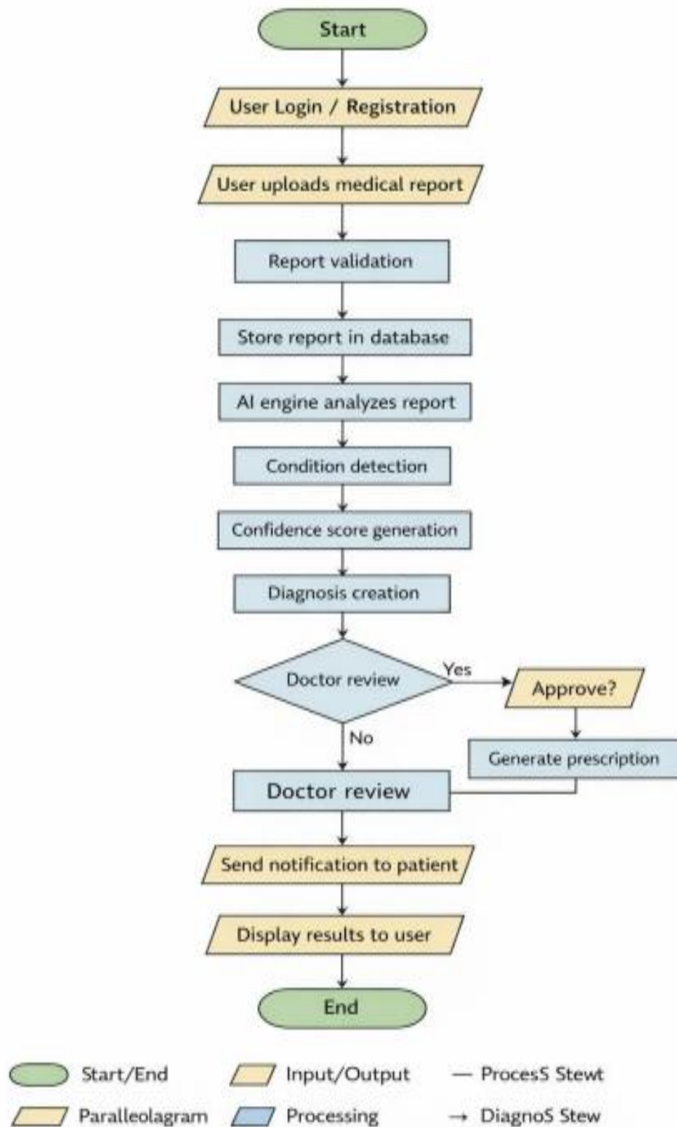
Figure 3.5: Flowchart of MedScan
