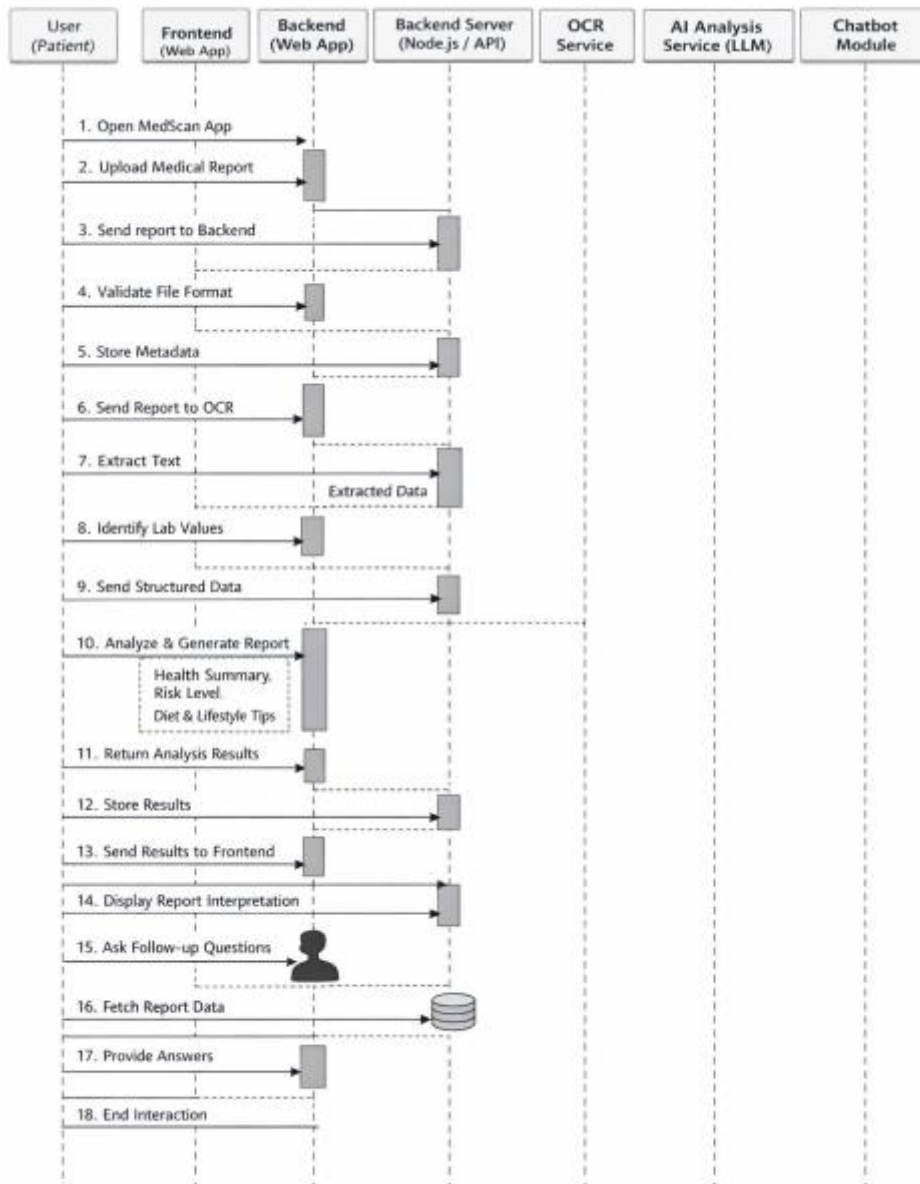
Figure 3.4: Sequence Diagram of MedScan
