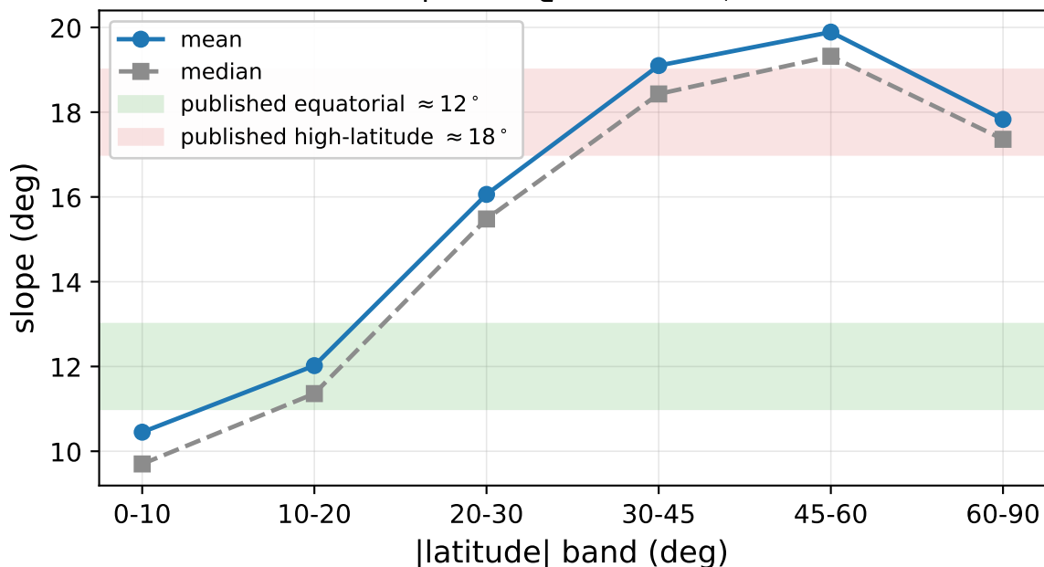
(a) Bennu latitudinal profile, \rho = 1.194 , N_f = 30\,561
