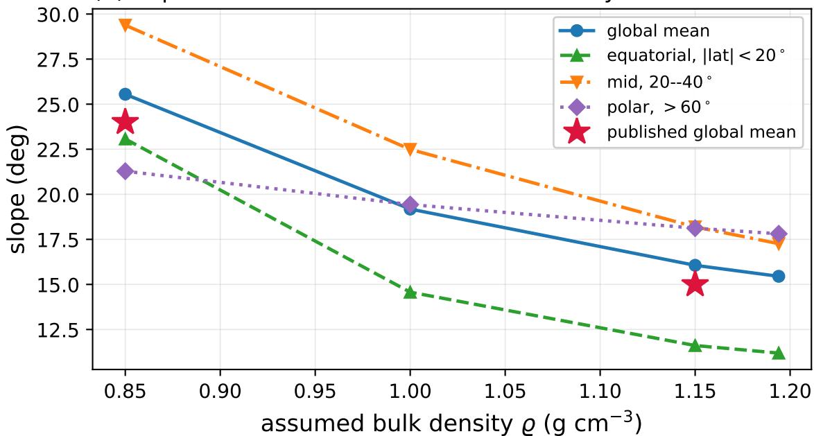
(b) dependence on the assumed bulk density
