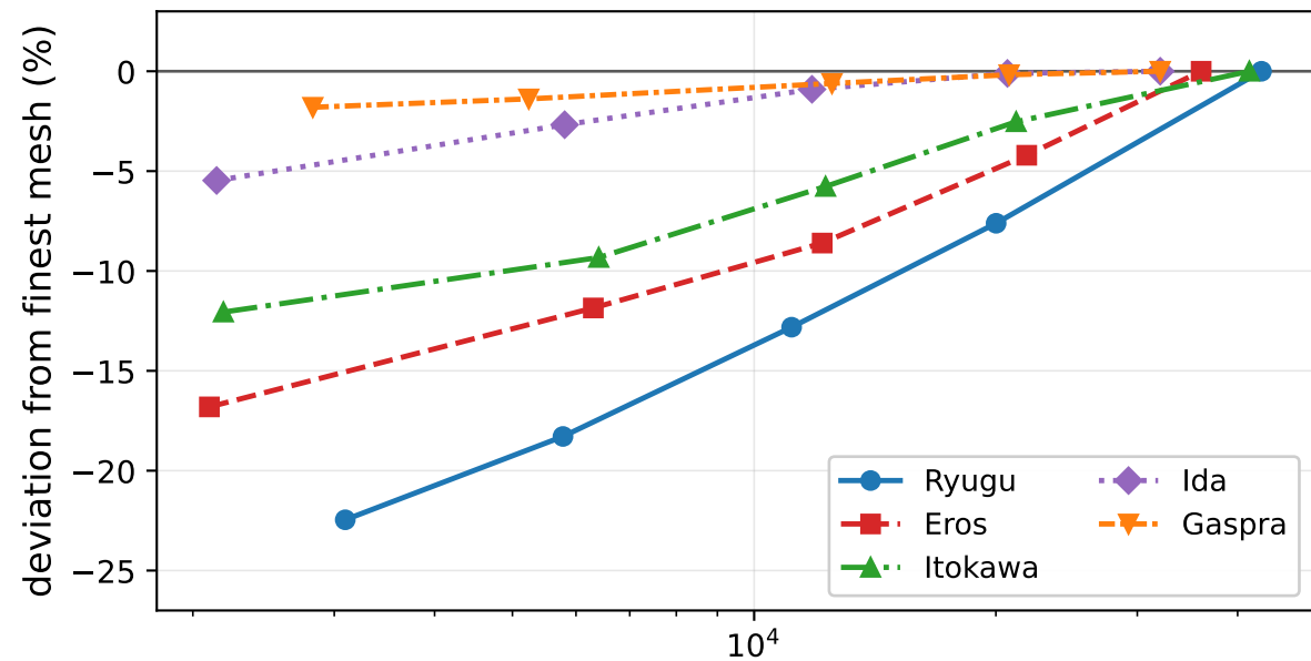
(a) area-weighted mean slope \bar{\theta}
