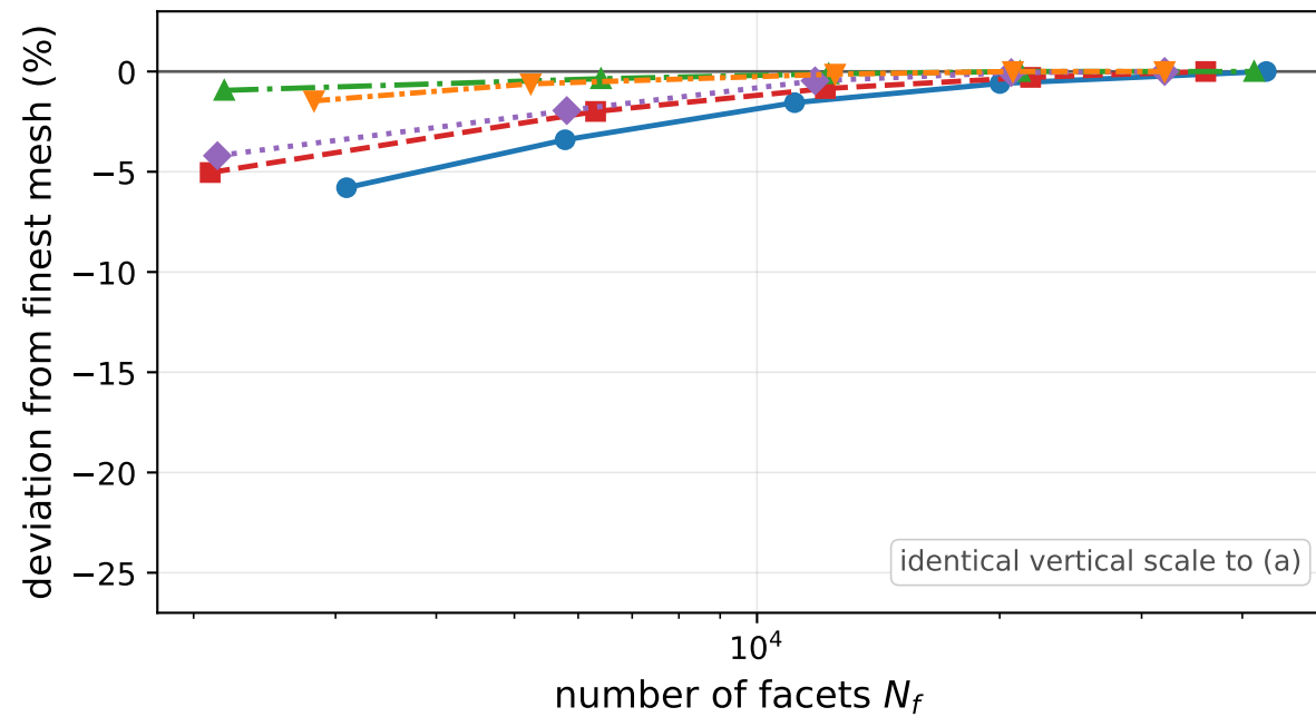
(b) normalized geopotential dispersion \tilde{\sigma}_U
