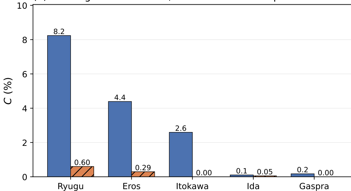
(b) convergence residual C , final refinement step
