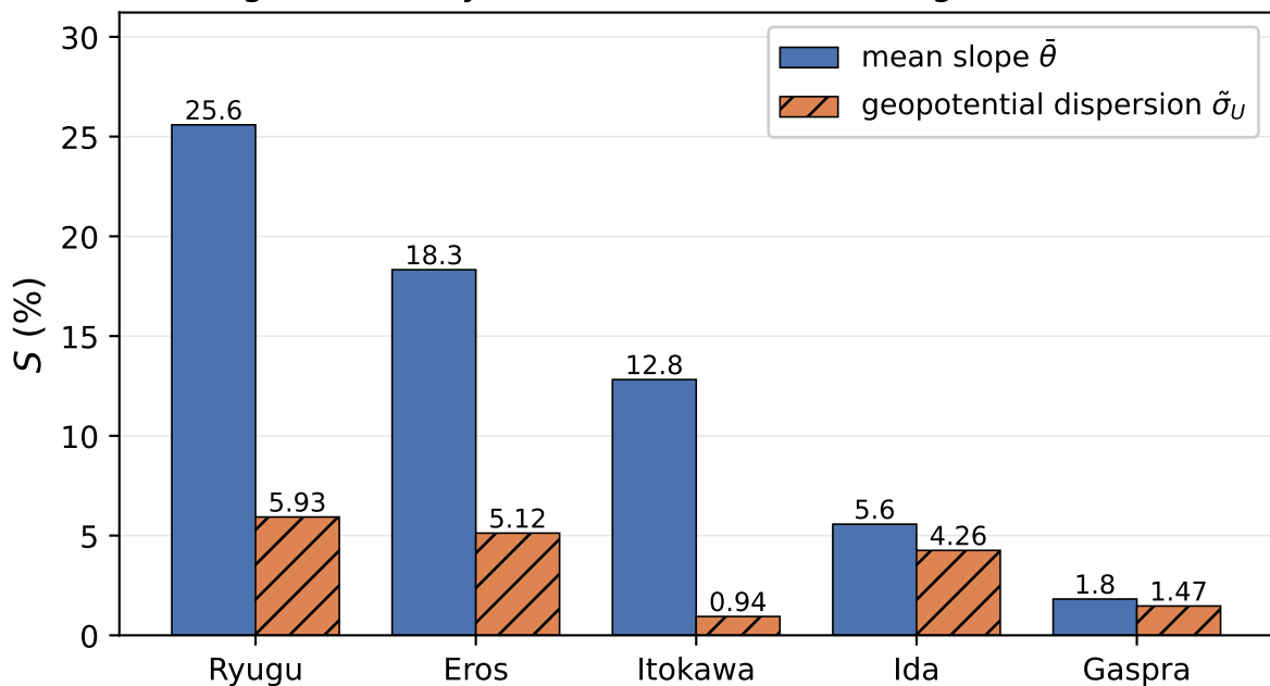
(a) range sensitivity S over the full mesh range
