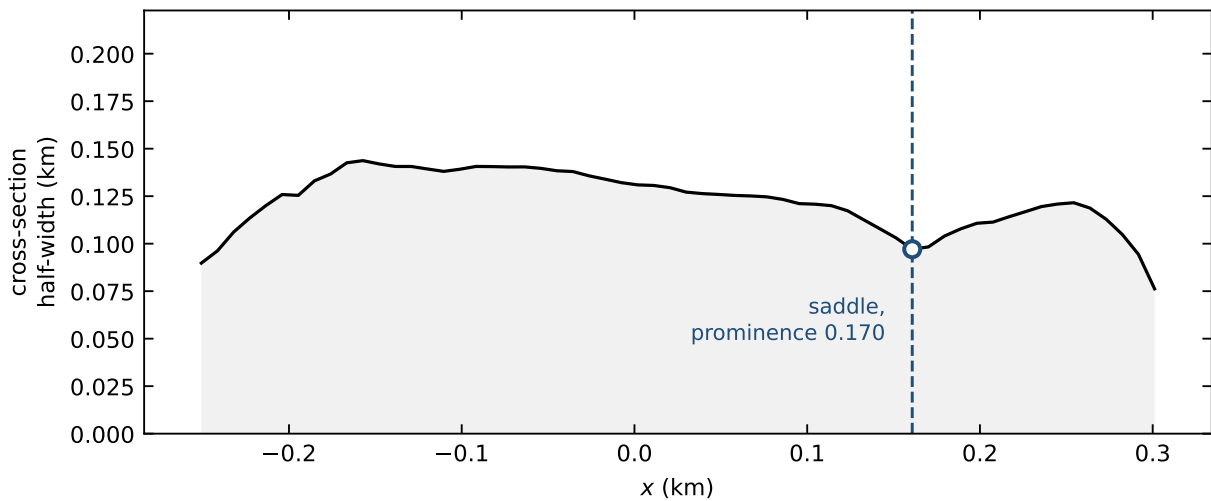
Itokawa — 1 of 3 local minima accepted
