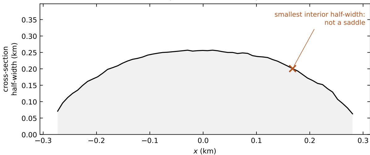
Bennu — no saddle accepted (3 local minima, prominence < 0.02)
